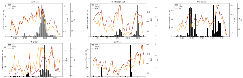
Figure F1: 50-day comparison of the FWI and HDWI indices over each study region with FRP overlaid.
