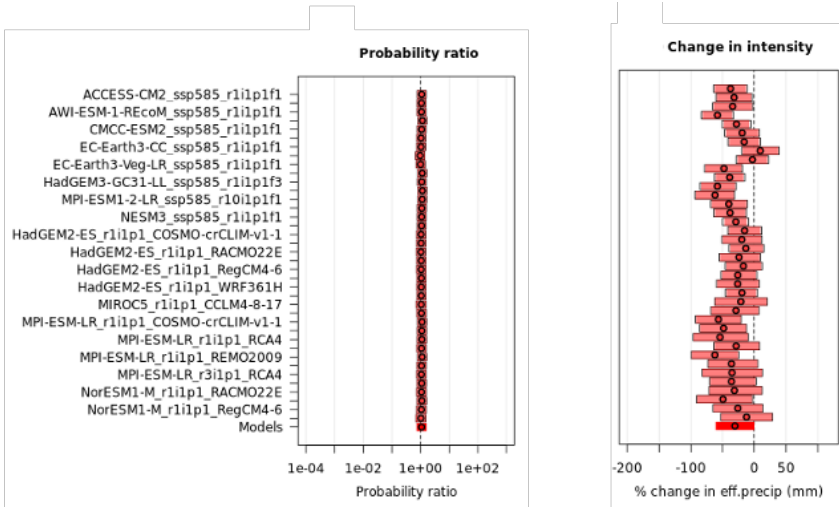
Figure A8: MAM eff precip synthesis from present day (+1.3°C) to +2.6°C
