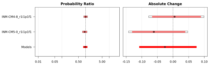
Figure C6: Maximum 7-day wind speed synthesis from present day (+1.3°C) to +2.6°C
