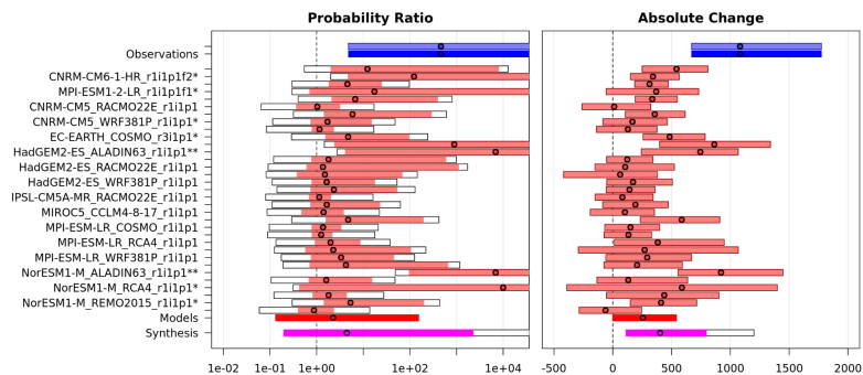
1080 Figure C3: Maximum 7-day VPD synthesis from pre-industrial to present day (+1.3°C)
