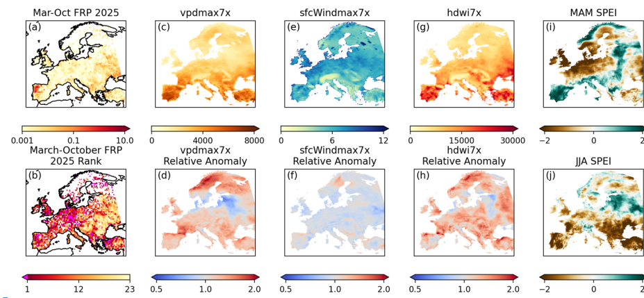
Figure 3: (a), the average FRP over the period March to October, 2025, according to the MODIS active fire product, and (b), the rank of 2025 MODIS FRP from Mar-Oct compared to other years since 2003. All statistics for subfigures c-h are calculated at the grid-cell level using ERA5-Land data: (c), The maximum annual 7-day rolling average of maximum daily vapour pressure deficit (vpdmax7x), and (d), the anomaly of vpdmax7x in 2025 relative to the climatology from 1990-2019. (e) the maximum annual 7-day rolling average of maximum daily windspeed (sfcWindmax7x), and (f), the anomaly of sfcWindmax7x in 2025 relative to the climatology from 1990-2019. (g) the maximum annual 7-day rolling average of the hot-dry-windy index – the product of maximum daily vapour pressure deficit and maximum daily windspeed (hdwi7x), and (h), the anomaly of hdwi7x in 2025 relative to the climatology from 1990-2019. Using ERA5-Land: (i), the standardised precipitation evapotranspiration index (SPEI) for spring (March-May) in 2025, calculated relative to 1990-2019. (j), the SPEI for summer (June-August) in 2025, calculated relative to 1990-2019.
