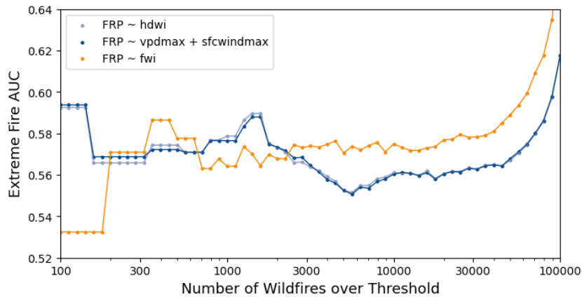
Figure F3: the predictive power of different variable sets in a Gamma distribution GLM with log-link function for classifying the N most extreme wildfires by FRP according to the area under the receiver operating curve statistic (AUC). A single variable HDWI model performs extremely similarly to a model with VPDmax and sfcWindmax accounted for separately. HDWI performs best at capturing the rarest and most extreme wildfires, similarly for the next most extreme wildfires (from the top 3000 to 300 FRP events) and worse for more moderate wildfire events (below the top 3000 class).
