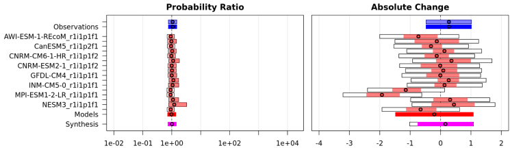
1045 Figure B5: Maximum 7-day wind speed synthesis from pre-industrial to present day (+1.3°C)
