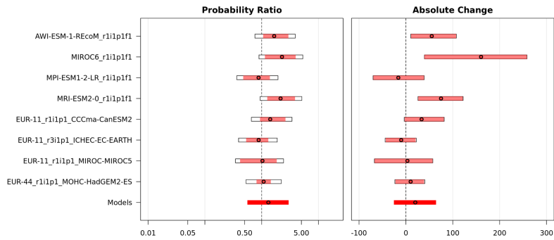
1040 Figure B4: Maximum 7-day VPD synthesis from present day (+1.3°C) to +2.6°C
