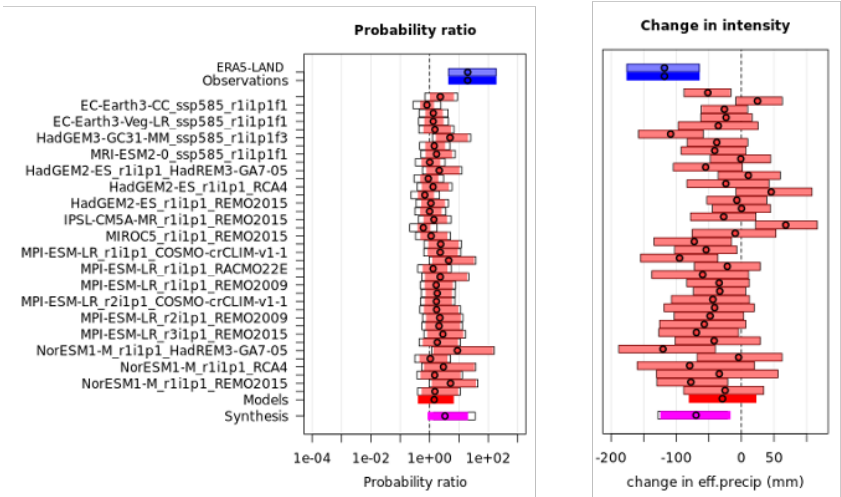
1105 Figure C9: JJA eff precip synthesis from pre-industrial to present day (+1.3°C)
