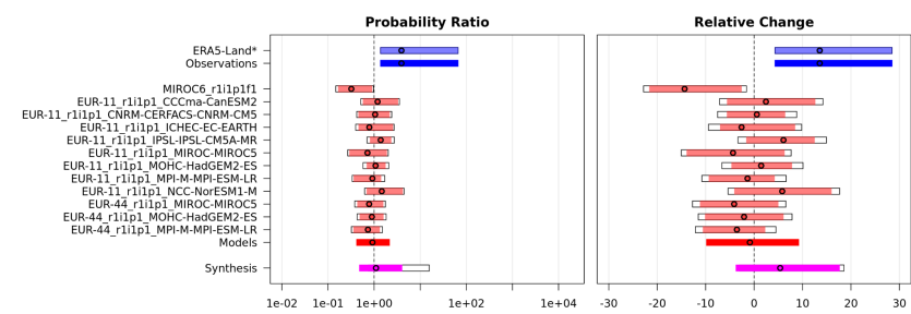
Figure B1: HDWI synthesis from pre-industrial to present day (+1.3°C)
