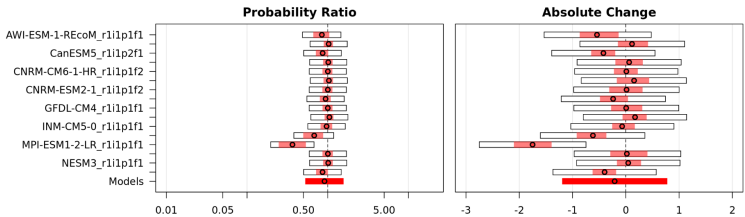
Figure B6: Maximum 7-day wind speed synthesis from present day (+1.3°C) to +2.6°C
