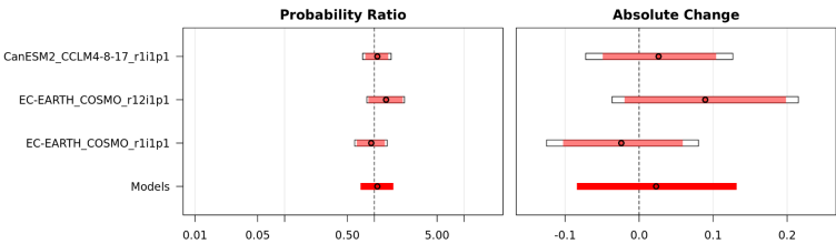
Figure E6: Maximum 7-day wind speed synthesis from present day (+1.3°C) to +2.6°C
