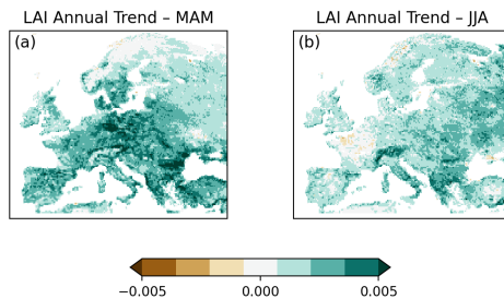
Figure 4: summary of the annual trend ( \text{yr}^{-1} ) at 0.5^\circ aggregated grid cells in (a) spring (March-May) and (b) summer (June-August) leaf area index (LAI) per a Theil-Sen estimator of the linear slope – using corrected LAI data from Ryu et al. (2018): 1982 to 2024.
