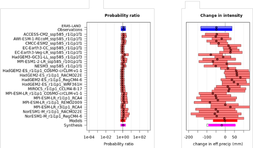
Figure A7: MAM eff precip synthesis from pre-industrial to present day (+1.3°C)
