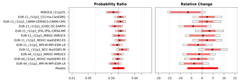
Figure B2: HDWI synthesis from present day (+1.3°C) to +2.6°C
