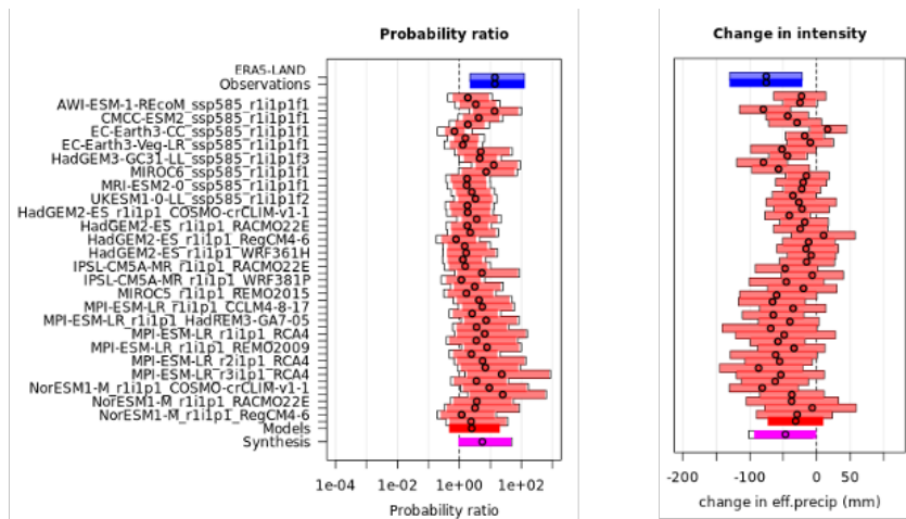
Figure A9: JJA eff precip synthesis from pre-industrial to present day (+1.3°C)
