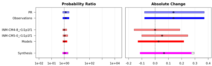
Figure C5: Maximum 7-day wind speed synthesis from pre-industrial to present day (+1.3°C)
