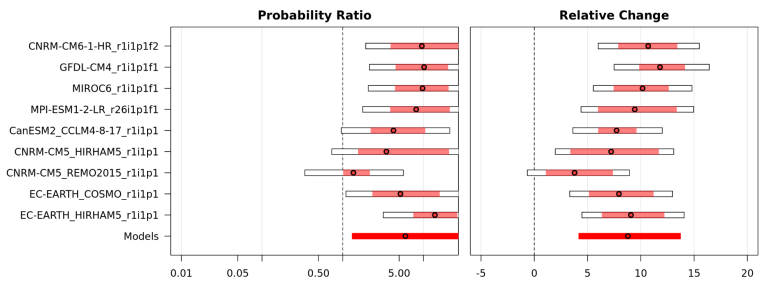
1160 Figure E2: HDWI synthesis from present day (+1.3°C) to +2.6°C
