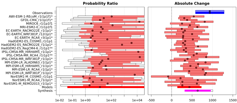
1165 Figure E3: Maximum 7-day VPD synthesis from pre-industrial to present day (+1.3°C)
