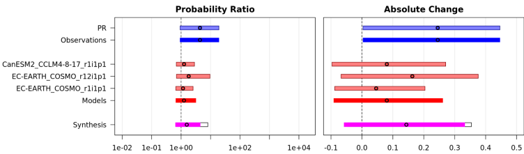
Figure E5: Maximum 7-day wind speed synthesis from pre-industrial to present day (+1.3°C)
