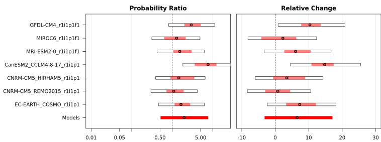
1075 Figure C2: HDWI synthesis from present day (+1.3°C) to +2.6°C
