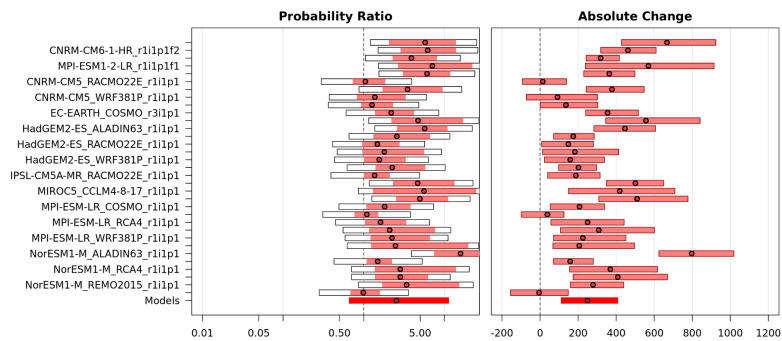
Figure C4: Maximum 7-day VPD synthesis from present day (+1.3°C) to +2.6°C
