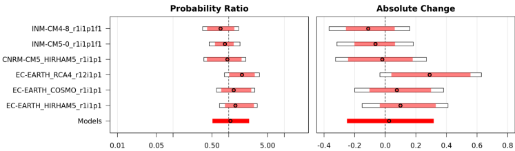
Figure A6: Maximum 7-day wind speed synthesis from present day (+1.3°C) to +2.6°C
