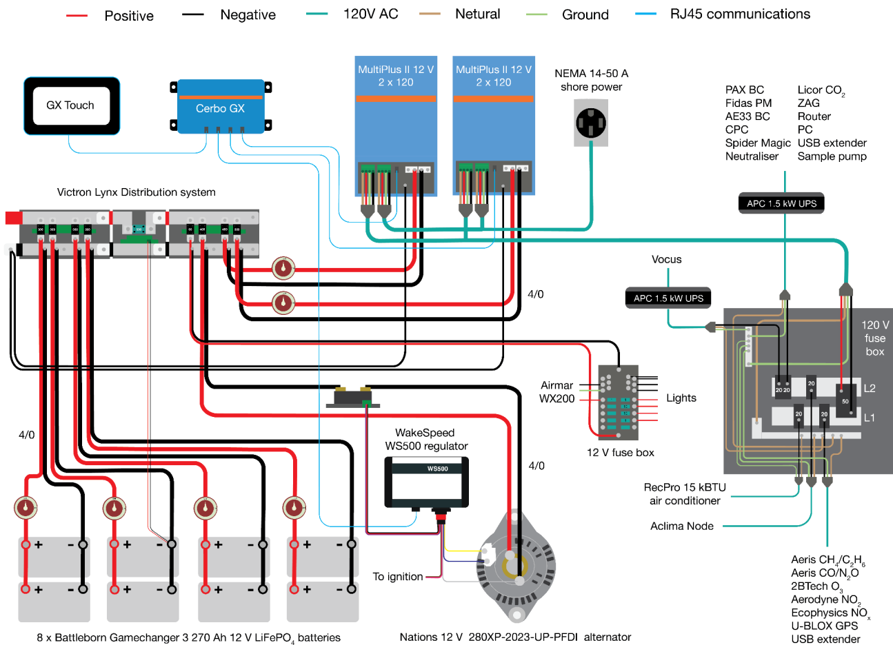
245 Figure 2: Complete electrical system wiring diagram for the CalMAPLab including the battery bank, busbar distribution and inverter system, as well as fuse box wiring, alternator charging and Victron communications.
