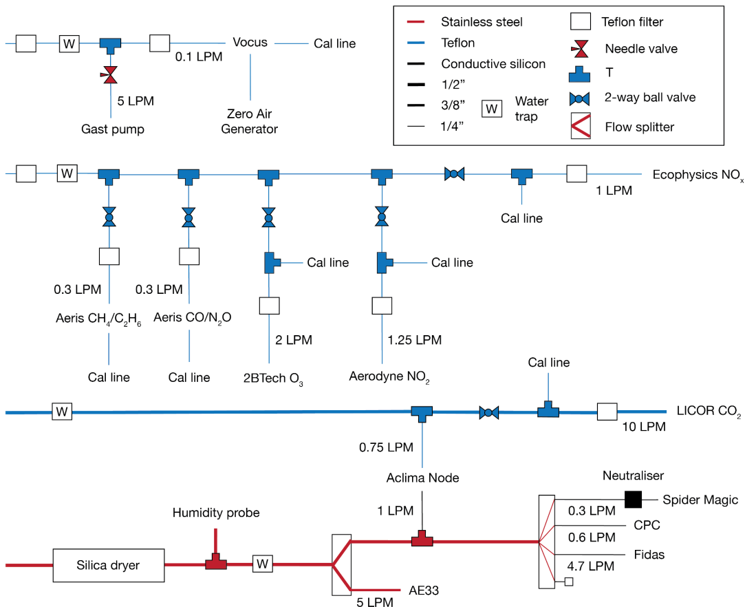
295 Figure 3: Schematic of the inlet configuration and flows for the three gas phase and singular particle phase sampling lines. Further details on each instrument are provided in Table 1.
