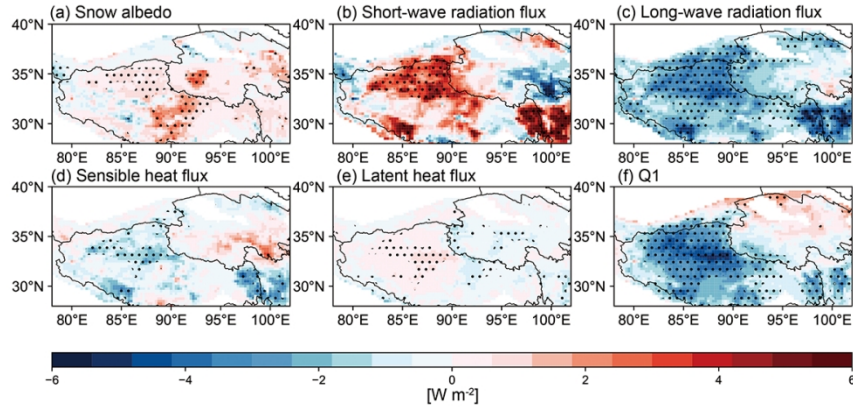
Figure 6. Anomalies for (a) snow albedo (dimensionless, multiplied by 100), (b) top net short-wave radiation flux ( W m^{-2} ), (c) top net long-wave radiation flux ( W m^{-2} ), (d) surface sensible heat flux ( W m^{-2} ), (e) surface latent heat flux ( W m^{-2} ), (f) total atmospheric column heat source ( W m^{-2} ) during winter over 1979-2021 obtained by regression upon normalized TPSC index. Dotted areas represent statistical significance with 95% confidence according to Student's t test.
