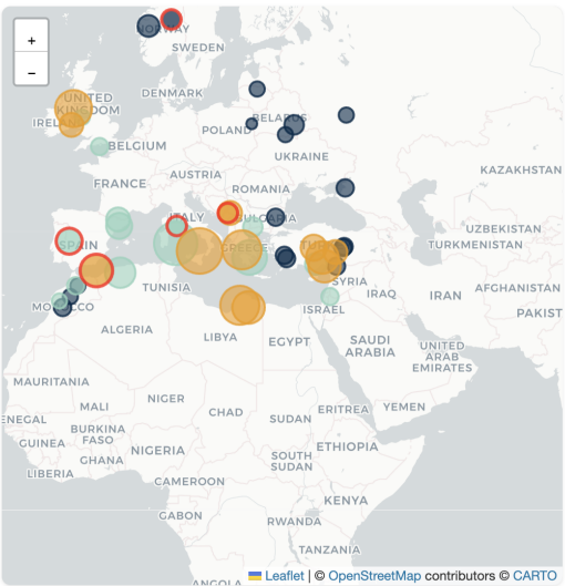
Figure A1. Real-time dashboard of the RHITA web tool. Screenshot from the RHITA website taken on 28 January 2026. The figure displays events affecting Europe between 14 and 28 January 2026. Small cold spell events are visible in northern and western Europe, while larger events are detected over southern Europe, particularly southern Italy.
