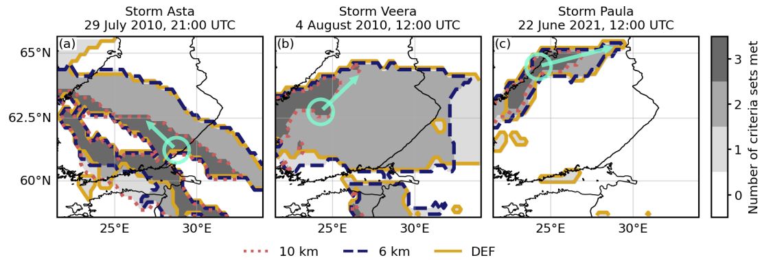
Figure 4. Areas satisfying each criteria set during the storms Asta (29 July 2010 at 21 UTC) in panel (a), Veera (4 August 2010 at 12 UTC) in panel (b) and Paula (22 June 2021 at 12 UTC) in panel (c). Shades of gray indicate how many of the three criteria sets are met in each grid cell. The areas satisfying the 10 km criteria set are outlined with red dotted lines, the 6 km criteria set with blue dashed lines and the DEF criteria set with gold solid lines. Aquamarine circles indicate the approximate location of the systems at the times of the analyses and arrows point to the approximate movement of the system during the following three hours.
