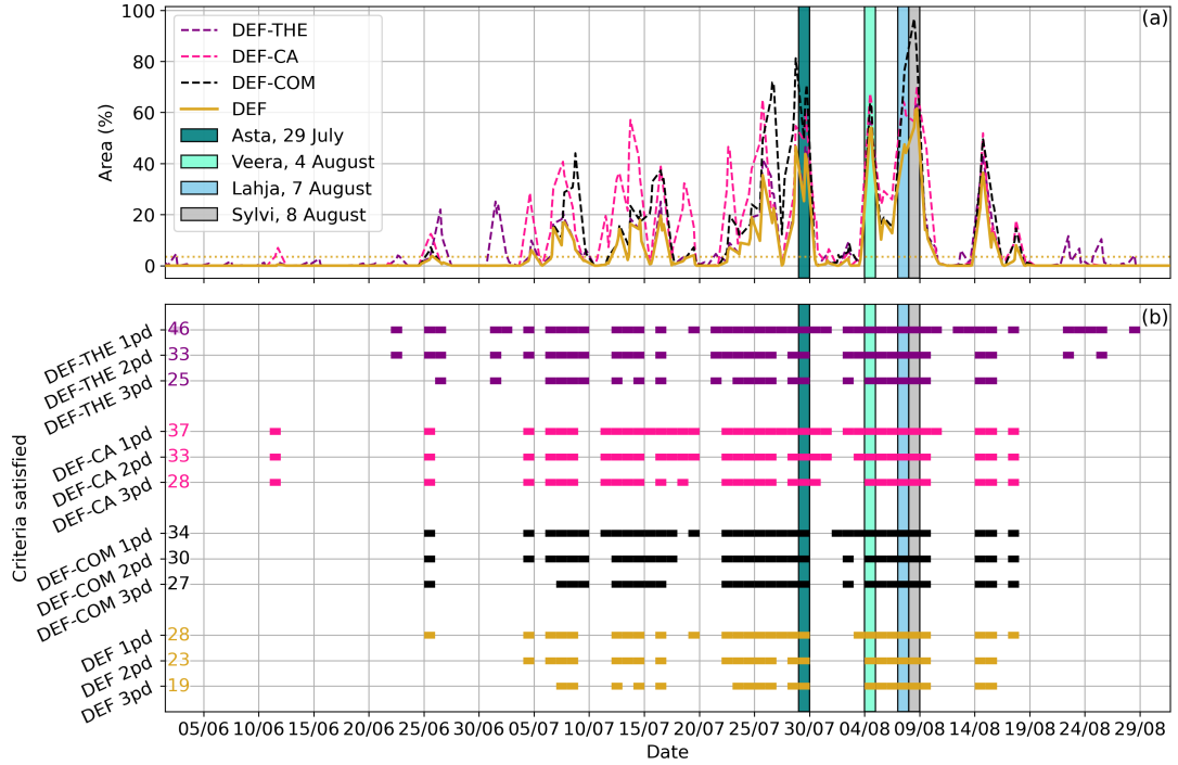
Figure 6. As in Fig. 5 but for combinations of criteria within the DEF criteria set, with the dashed lines representing the DEF criteria set excluding the 850 hPa \theta_E \geq 325 K condition (DEF-THE, purple), CAPE \geq 250 J kg -1 condition (DEF-CA, pink) and combined shear condition (DEF-COM, black). The gold solid line shows the full DEF criteria set (DEF) as a reference.
