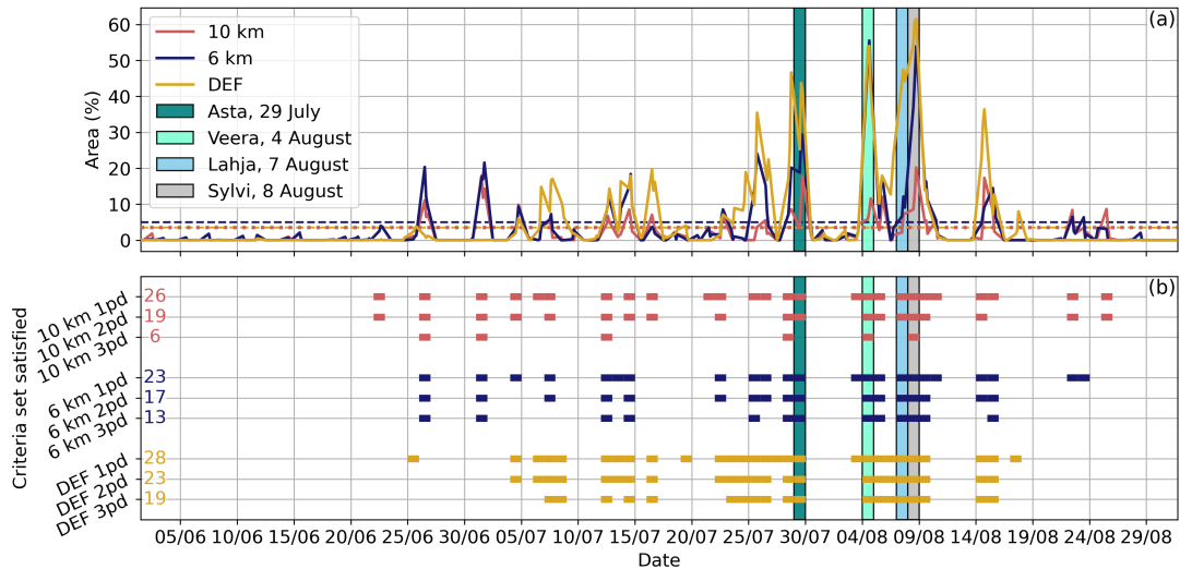
Figure 5. Performance of the criteria sets during the summer of 2010. Vertical bars in both panels indicate days when derechos occurred. Panel (a) shows the fraction (%) of the grid area where each criteria set is satisfied. The red line represents the 10 km criteria set, the blue line the 6 km criteria set, and the gold line the DEF criteria set. Data includes three time steps per day (12, 15, and 18 UTC), as described in Sect. 2.4. Horizontal lines illustrate the area demands for each criteria set: 5 % for the 6 km criteria set (blue, dashed) and 3.5% for both the 10 km (red, dashed) and DEF criteria sets (gold, dotted). Panel (b) presents the favorable days throughout the summer for each criteria set, with conditions satisfied once per day (1pd), twice per day (2pd) and at all three times per day (3pd), illustrated with bold lines. Total number of favorable days for each category is indicated on the left side of the panel.
