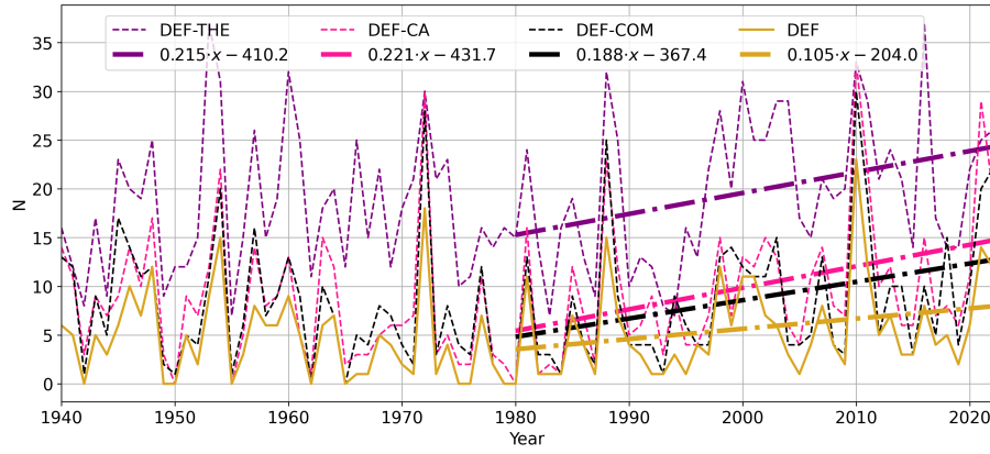
Figure 8. Similar to Fig. 7 but for the same criteria combinations within the DEF (2pd) criteria as in Fig. 56. The corresponding linear regression lines for the 1980–2022 period are drawn with dash-dotted lines.
