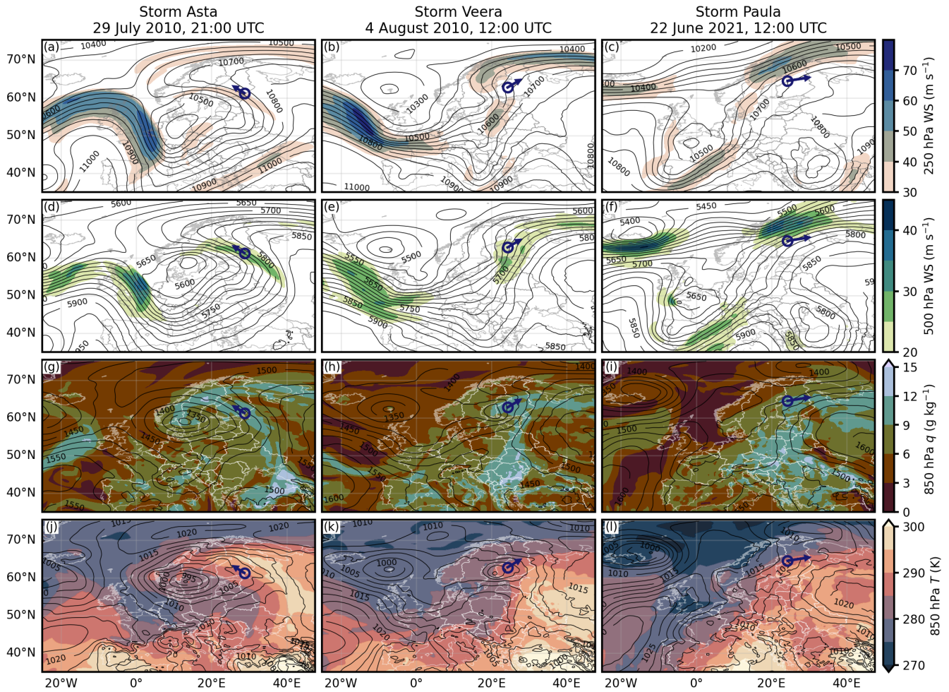
Figure 2. Synoptic-scale situation pattern during the storms Asta (29 July 2010 at 21 UTC) in the left column (panels a, d, g and j ), Veera (4 August 2010 at 12 UTC) in the left-center column (panels a, e, b, e, h and g, k ) and Paula (22 June 2021 at 12 UTC) in the right column (panels b, d, c, f, i and h, l ). Panels (a-b) (a-c) show wind speed (WS, shading starting from 30 \text{ m s}^{-1} ) and geopotential height at 250 hPa, (e-d) (d-f) wind speed (WS, shading starting from 20 \text{ m s}^{-1} ) and geopotential height at 500 hPa, (e-f) (g-i) specific humidity ( q , shading) and geopotential height (black contours) at 850 hPa, and (g-h) (j-l) temperature ( T ) at 850 hPa (shading) and mean sea level pressure (MSLP, black contours). In all panels, blue circles indicate the approximate location of the systems at the times of the analyses and arrows point to the approximate movement of the system during the following three hours.
