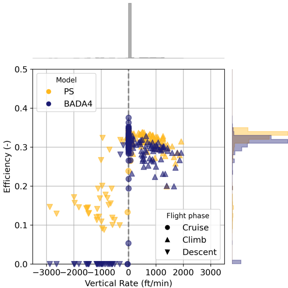
Figure A5. Scatter plot of overall engine-propulsion efficiencies against the vertical rate at the scanning time of the satellite, coloured according to the model used. The histograms on the vertical axis show the distribution of efficiencies per model, and those on the horizontal axis show the distribution of vertical rates.
