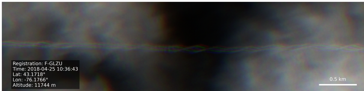
Figure D3. Contrail observed in Sentinel-2 imagery illustrating the occurrence of the Crow instability (Crow, 1970).
