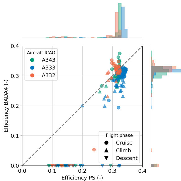
Figure A4. Scatter plot of overall engine-propulsion efficiency in Poll-Schumann and BADA 4.2 at the scanning time of the satellite. Colour indicates IAGOS aircraft type, marker indicates flight phase. Histograms show the distribution of engine-propulsion efficiencies shown with values scaled per aircraft type.
