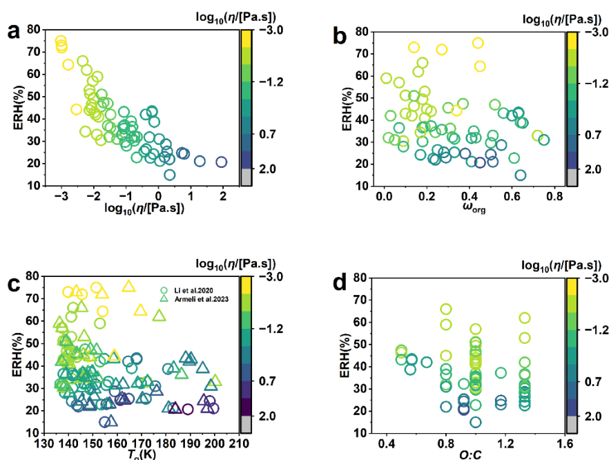
Figure 1. Relationships between the ERH of organic-inorganic mixed aerosols. (a) the logarithm of viscosity ( \log_{10}(\eta/[\text{Pa.s}]) ), (b) the organic mass fraction ( \omega_{\text{org}} ), (c) the glass transition temperature ( T_g(\omega_{\text{org}}) , K) calculated using the methods of Li et al. (Li et al., 2020) and Armeli et al. (Armeli et al., 2023), respectively, and (d) O:C ratio. The color bar denotes the aerosol viscosity in ( \log_{10}(\eta/[\text{Pa.s}]) ).
