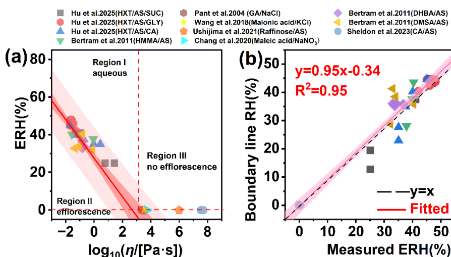
Figure 3. (a) Comparison between the validation dataset and viscosity-ERH boundary framework (Eq. 5), showing three distinct regions in viscosity–humidity space: Region I (aqueous state), Region II (efflorescence-favorable conditions), and Region III (non-efflorescence or highly viscous state). (b) Comparison between experimentally measured ERH values and the boundary line RH values derived from the viscosity–humidity relationship. The black dashed line denotes the y = x reference line, and the red line represents the linear regression fit to the data, along with the corresponding coefficient of determination, R^2 = 0.95 . The pale pink shading represents the 95% confidence interval. DEMA represents Diethyl malonic acid, DMSA represents 2,2-Dimethyl succinic acid, DMGA represents 3,3-Dimethyl glutaric acid, HMMA represents DL-4-Hydroxy-3-methoxymandelic acid and DHBA represents 2,5-Dihydroxybenzoic acid, CA represents citric acid, SUC represents Sucrose, GA represents glutaric acid, HXT represents 1,2,6-hexanetriol.
