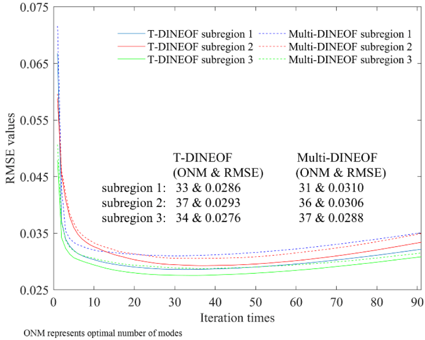
15 ONM represents optimal number of modes 16 Fig. 17 Distributions of RMSE values at the cross-validation pixels for T-DINEOF and 17 Multi-DINEOF across three subregions during the iterative process.
