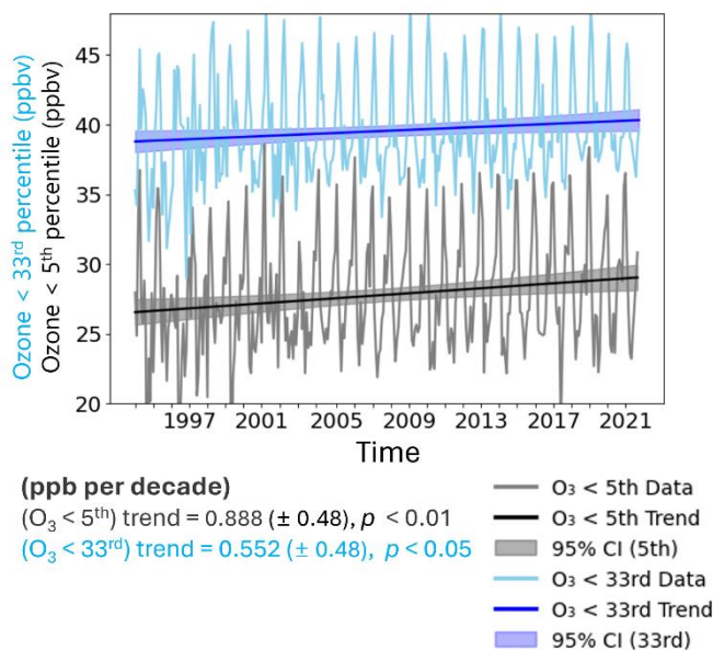
(c) In-situ O_3 – Clean O_3 Western North America (25 - 55N, 130 - 90W)
