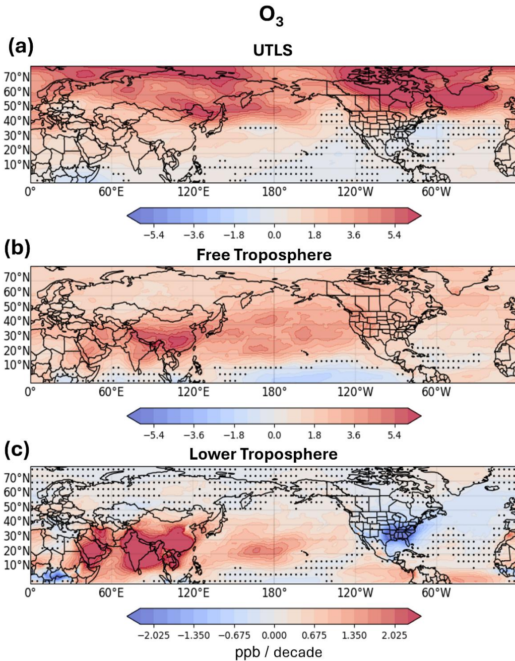
365 Figure 7. GMI O 3 trend (ppb decade -1 ) in the (a) UTLS (244.88–176.93 hPa), (b) free troposphere (700–288.88 hPa), and (c) lower troposphere (725–985 hPa) calculated from 1994 and 2019. The dots on the maps represent the grid cells with a lower confidence value ( p -value \geq 0.05 ). The pressure shown here represents the midpoint of each GMI model level.
