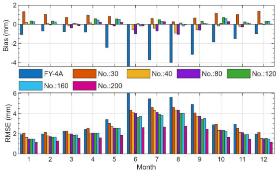
440 Figure 9. Comparison of the Accuracy of FY-4A PWV and Their Calibrated Versions Using Different Models Based on GNSS Validation.
