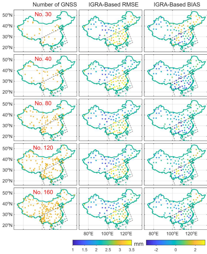
310 Figure 5. Spatial distribution of validation accuracy for different models using IGRA stations.
