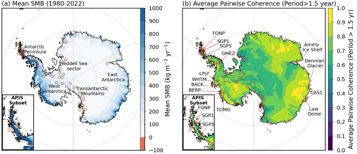
Figure 2: (a) Mean annual SMB averaged across the seven SMB models for the common period 1980-2022, shown on a 2 km interpolated grid. GPS site locations are shown by brown circle and major Antarctic regions, as referred to in the text, are labelled. (b) Average pairwise SMB model coherence (unitless) at low-frequencies (periods greater than 1.5 years), computed on the same 2 km grid. GPS site locations are shown by brown circles and site names or regions discussed in the text are annotated.
