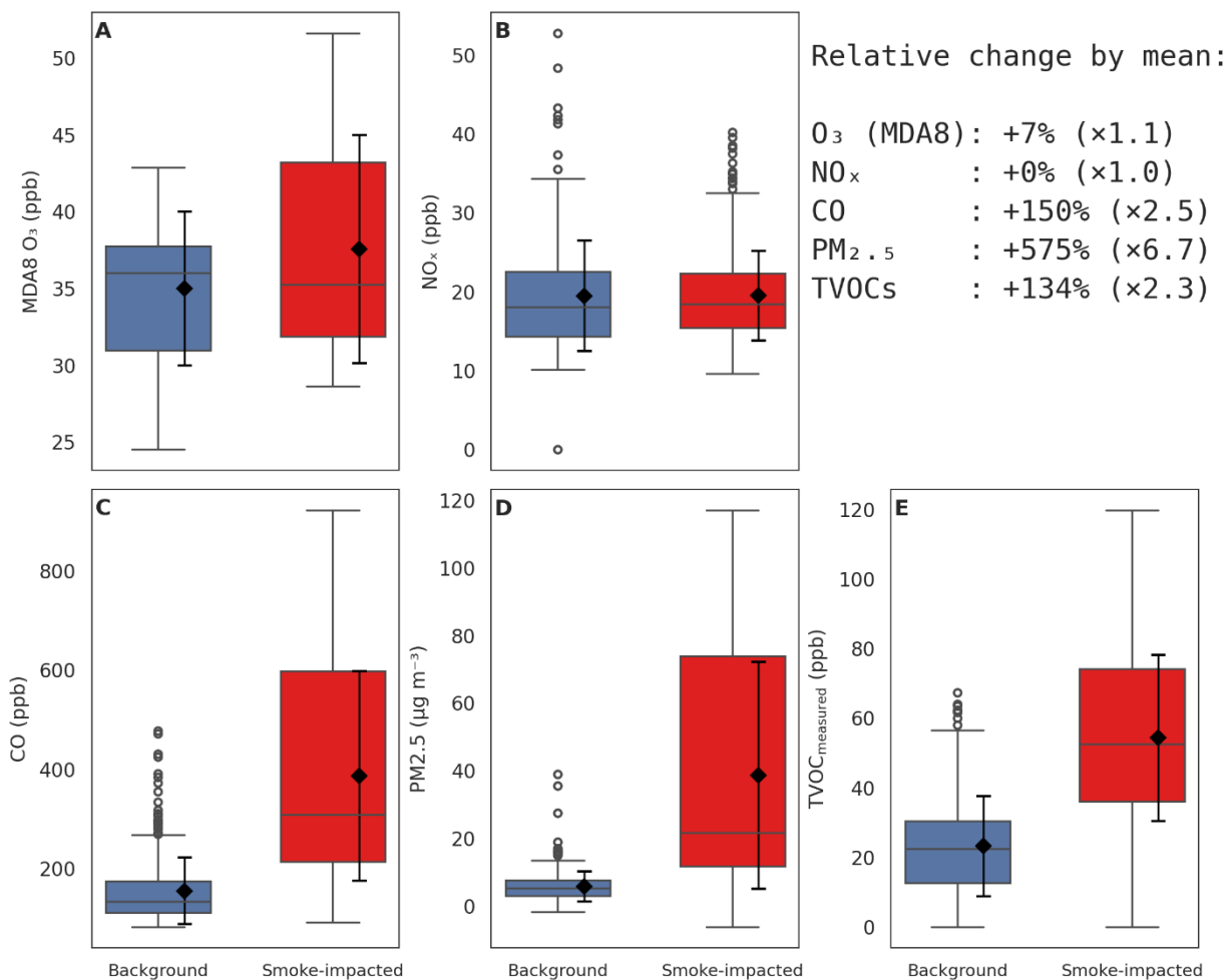
Figure 4. Enhanced surface-level pollutant concentrations during smoke-impacted periods. Boxplots show (A) maximum daily 8-hour average ozone (MDA8 \text{O}_3 ) and hourly concentrations of (B) nitrogen oxides ( \text{NO}_x ), (C) carbon monoxide (CO), (D) fine particulate matter ( \text{PM}_{2.5} ), and (E) total measured volatile organic compounds (TVOCs) during smoke-impacted (red) and background (blue) periods in Missoula, Montana, during September 2020. Boxes represent interquartile ranges (25th–75th percentiles) with medians shown as center lines; whiskers extend to 1.5\times the interquartile range. Black diamonds and error bars indicate mean \pm standard deviation for each group. The right-hand summary block lists mean enhancement factors (smoke-impacted \div background) for each pollutant.
