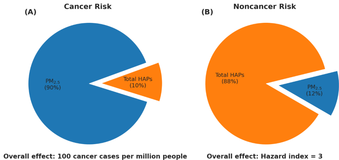
460 Figure 7. Chronic health-risk from fine particulate matter (PM 2.5 ) and hazardous air pollutants (HAPs). (A) Estimated excess cancer risk (cases per million people) attributed to ambient PM 2.5 versus all combined HAPs. (B) Noncancer hazard index (HI) attributed to ambient PM 2.5 versus combined HAPs. In each panel, slices are exploded for clarity, and labels show the percentage of total risk contributed by each component. The bottom annotation reports the overall risk magnitude: total cancer cases per million for panel A and HI for panel B. 465
