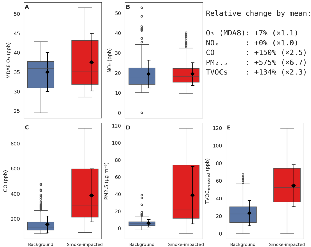
Figure 4. Enhanced surface-level pollutant concentrations during smoke-impacted periods. Boxplots show (A) maximum daily 8-hour average ozone (MDA8 O 3 ) and hourly concentrations of (B) nitrogen oxides (NO x ), (C) carbon monoxide (CO), (D) fine particulate matter (PM 2.5 ), and (E) total measured volatile organic compounds (TVOCs) during smoke-impacted (red) and background (blue) periods in Missoula, Montana, during September 2020. Boxes represent interquartile ranges (25th–75th percentiles) with medians shown as center lines; whiskers extend to 1.5× the interquartile range. Black diamonds and error bars indicate mean \pm standard deviation for each group. The right-hand summary block lists mean enhancement factors (smoke-impacted \div background) for each pollutant.
