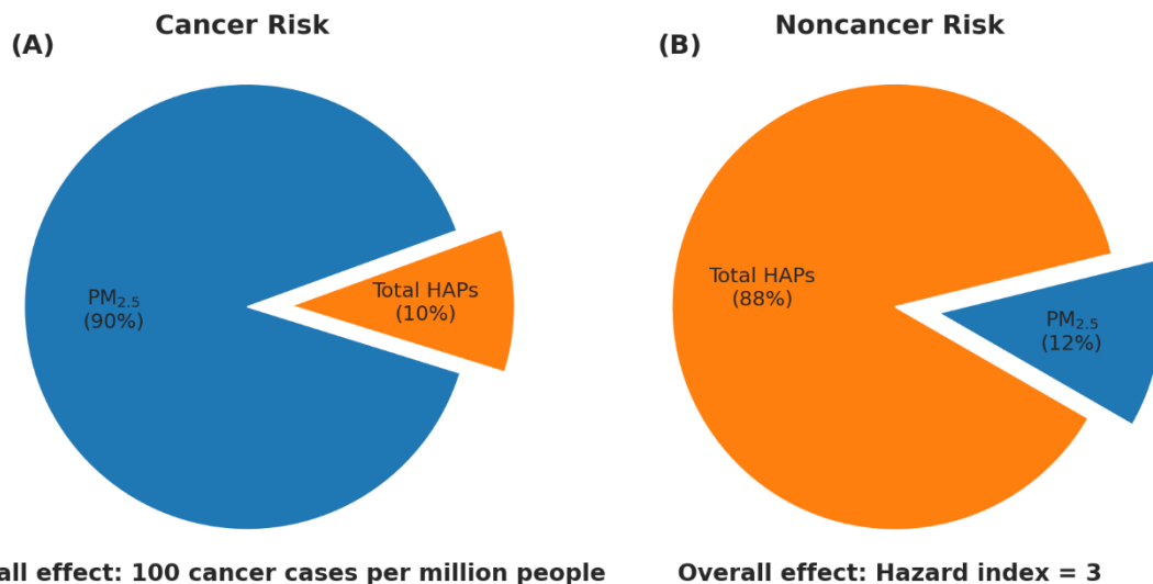
Figure 7. Chronic health-risk from fine particulate matter (PM 2.5 ) and hazardous air pollutants (HAPs). (A) Estimated excess cancer risk (cases per million people) attributed to ambient PM 2.5 versus all combined HAPs. (B) Noncancer hazard index (HI) attributed to ambient PM 2.5 versus combined HAPs. In each panel, slices are exploded for clarity, and labels show the percentage of total risk contributed by each component. The bottom annotation reports the overall risk magnitude: total cancer cases per million for panel A and HI for panel B.
