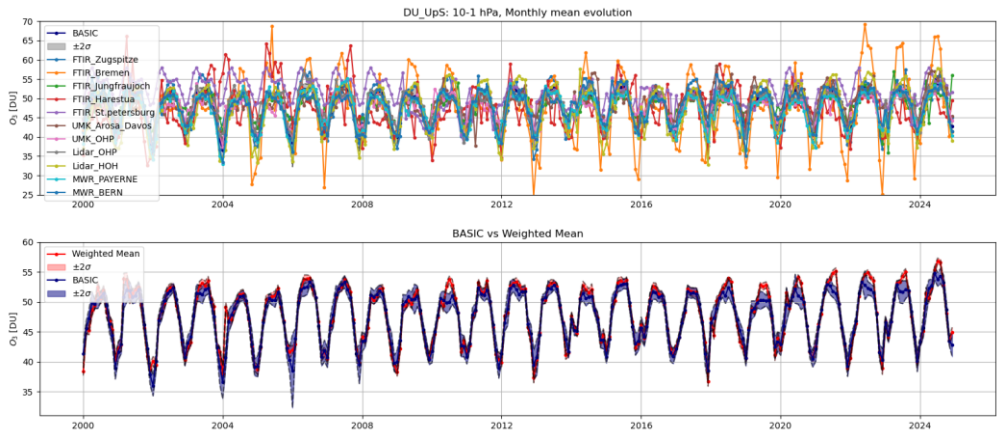
635 Figure 7: Time series for regional group central Europe, in the Upper Stratosphere (UpS). Top: time series of the group members, plotted with BASIC in blue and its uncertainty in grey. Bottom: comparison between BASIC in blue, with 2 uncertainties in blue, and the Weighted mean in red, with 2 uncertainties in red.
