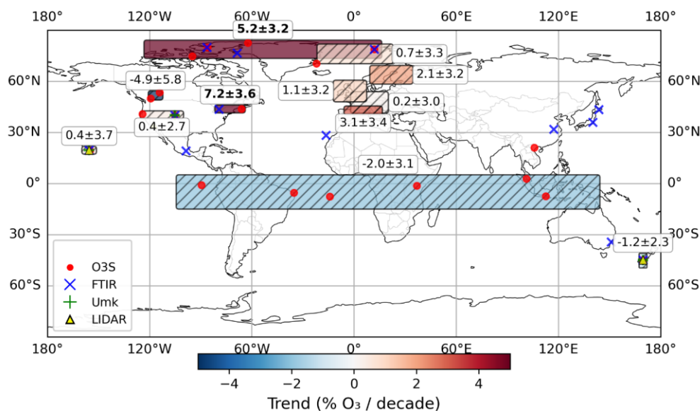
Figure 23: Same as figure 20 for layer UTL5
