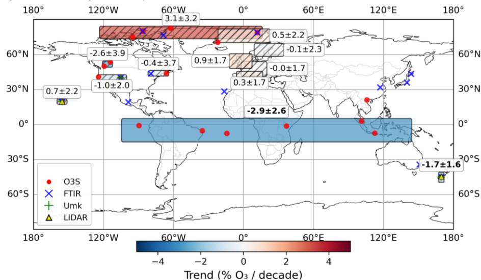
Figure 22: Same as figure 20 for layer LS
