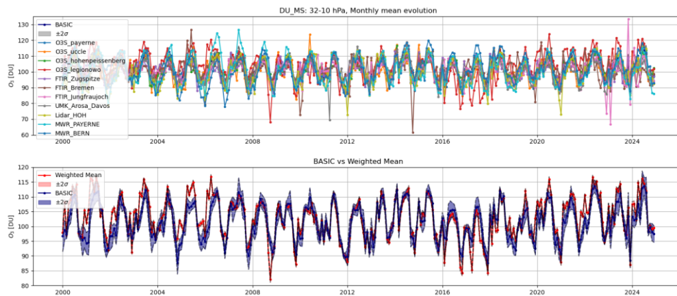
640 Figure 8: Same as Fig. 7 for the Middle Stratosphere (MS).
