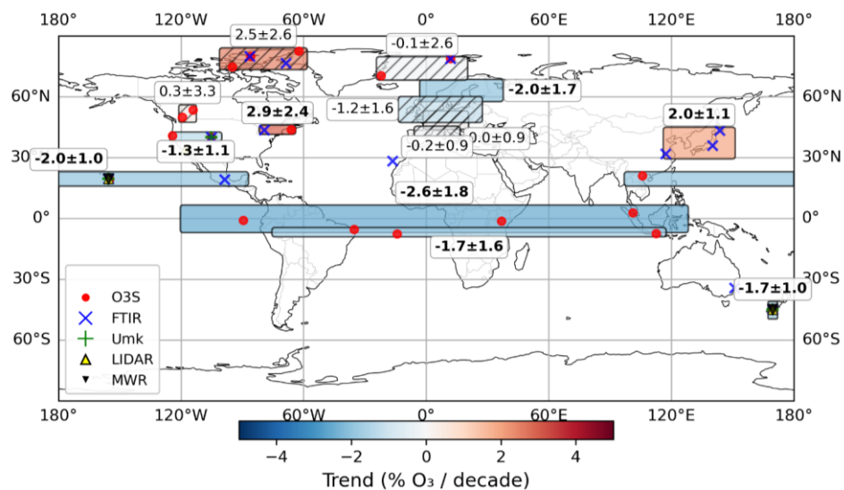
Figure 21: Same as figure 20 for layer MS
