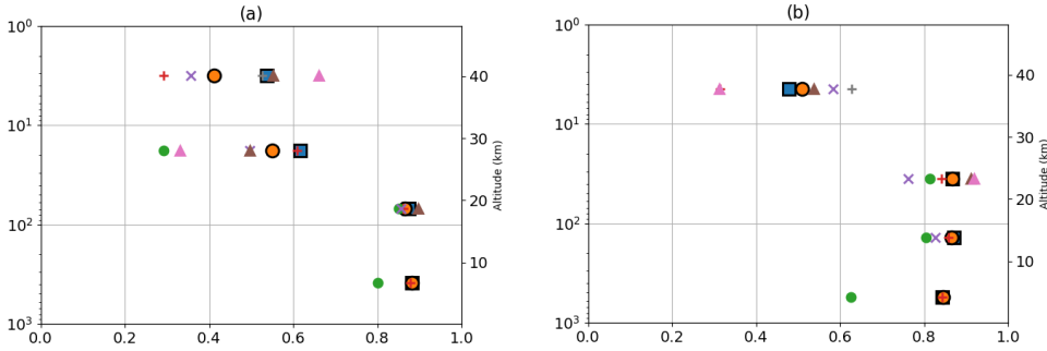
Figure 19: Adjusted R2 for BASIC, the weighted mean and the datasets of the Lauder group for (a) sPC and (b) aPC . Legends are similar to those of figures 17 and 18.
