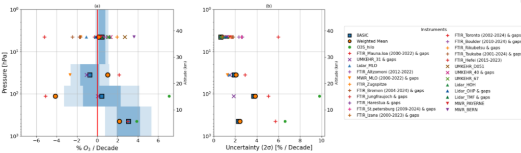
Figure 15: Same as 14 for the aPC of the group Hawaii.
