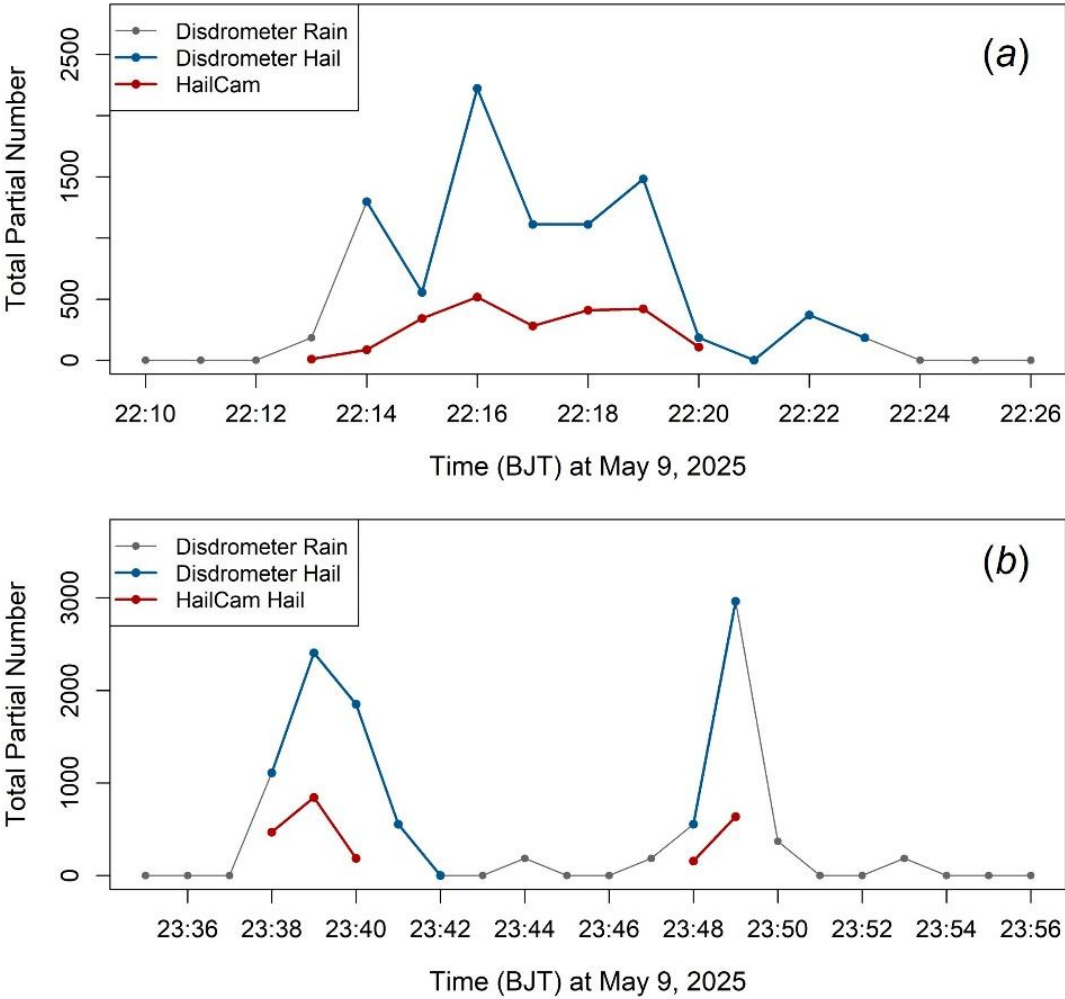
281 282 Figure 6: Temporal evolution of total particle number with diameters \geq 5 mm are considered. detected by the OTT Parsivel 2 283 disdrometer and HailCam during two hail episodes on 9 May 2025. (a) First hail episode (22:13–22:20 BJT) and (b) second hail 284 episode (23:38–23:49 BJT). The disdrometer data are disaggregated into rain (grey) and hail (blue) components based on the 285 instrument's classification algorithm, while HailCam measurements (red) represent hail particles with equivalent diameters \geq 5 mm. 286 Note the different scales on the y-axes between panels (a) and (b).
