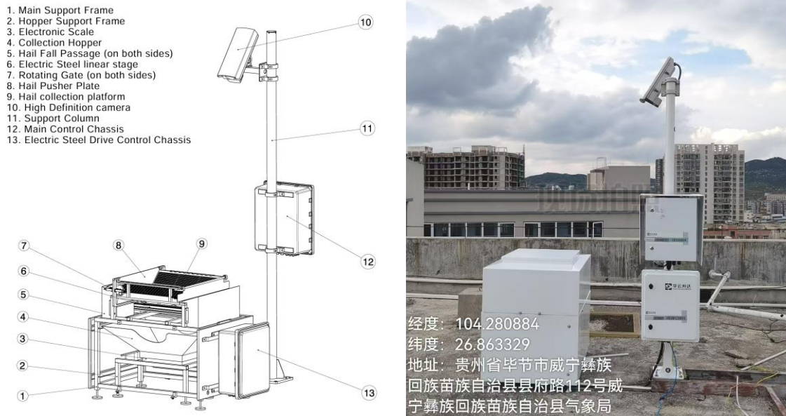
87 88 89 Figure 1: The major components of the hail observation device (left panel). Note: An electronic scale is installed beneath the 90 collection tray for experimental mass validation (not used in the current automated algorithm). Photo of the HailCam deployed at 91 the Weining Hail Suppression Experimental Base.
