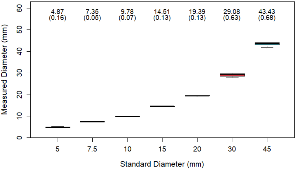
246 247 Figure 4: Boxplot of measured hailstone diameters from HailCam versus seven standard reference sizes (5–45 mm). For each size 248 class, 500 artificial ice spheres were individually introduced into the collection tray and automatically sized by the imaging system. 249 The mean measured diameter and standard deviation (in parentheses) are labelled above each box.
