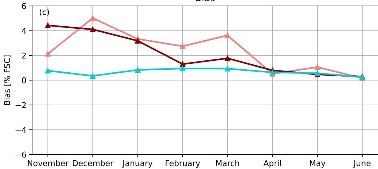
Bias
