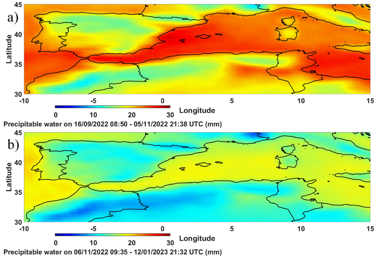
Figure 2. Precipitable water derived from IASI products during the wet period (16 September to 5 November 2022) and the dry period (6 November 2022 to 12 January 2023), as observed during the WaLiNeAs field campaign.
