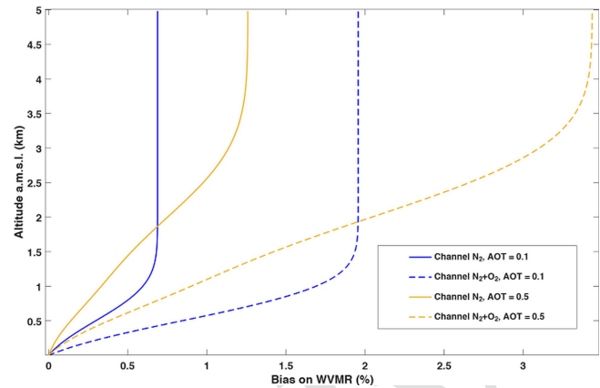
Figure B1. Bias on the lidar-derived water vapor mixing ratio due to the differential aerosol transmission between the water vapor Raman channel and the roto-vibrational nitrogen (N 2 ) or the rotational (N 2 + O 2 ) channels. Two typical aerosol loads encountered during the field campaign are considered: (i) an aerosol optical thickness (AOT) of 0.1 with an Ångström exponent of 1.5 (shown in blue) and (ii) an AOT of 0.5 with an Ångström exponent of 0.5 (shown in orange), which corresponds to the presence of dust aerosols.
