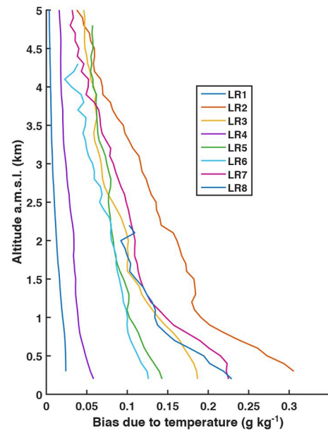
Figure B2. Vertical profiles of the maximum bias due to temperature variations for each lidar site (LR1 to LR8; see Table 1). The vertical profile of the water vapor mixing ratio considered is that shown in Fig. 4c.
