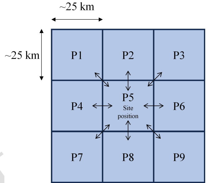
Figure 3. IASI pixels selected for comparison with lidar measurements. The central pixel includes the location of the lidar site. The horizontal resolution is 25 \text{ km} \times 25 \text{ km} for the water vapour product.
