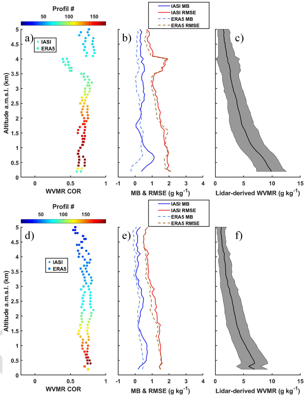
Figure 5. Synthesis of the statistical coefficients for the Toulon and Ajaccio lidar stations (RL6 and RL8) when comparing lidar measurements with IASI and ERA5 products. Wet conditions are illustrated in panels (a)–(c), while dry conditions are shown in panels (d)–(f). The vertical profiles show: (a, d) the correlation coefficient (COR); (b, e) the mean bias (MB, lidar – IASI and lidar – ERA5) and the root mean square error (RMSE); (c, f) the mean water vapour mixing ratio (WVMR) profile of all the overpasses of IASI. The contributions of aerosols and temperature to the bias are not considered.
