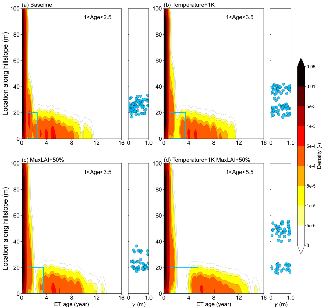
Figure 7. Source regions of particles contributing to December ET in the lower 20 m zone of the hillslope for selected age ranges under different ET-forcing scenarios. Left panels show the corresponding ET age distributions as a function of distance along the hillslope. Blue rectangles indicate the selected age intervals used to identify the particle populations shown in the right panels. Right panels show the inferred source locations of these ET-contributing particles in the x–y domain, where x represents distance along the hillslope and y represents the across-slope direction.
