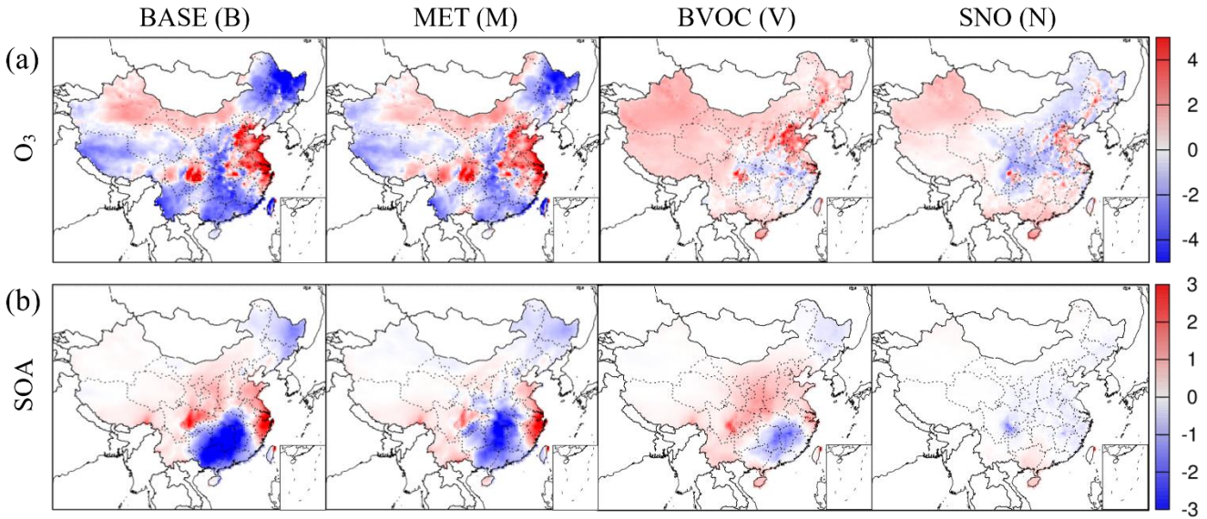
195 Figure 3. (a) Simulated differences in O 3 concentrations for BASE22–BASE21 (labeled ‘B’), BASE22–MET22 (labeled ‘M’), BASE22–BVOC22 (labeled ‘V’) and BASE22–SNO22 (labeled ‘N’). These scenarios represent the total differences between 2021 and 2022 (B), the contribution of meteorology (M), weather-driven BVOC (V) and SNO (N) emission changes, respectively (Units: ppb). (b) Same as (a) but for SOA (units: μg m -3 ).
