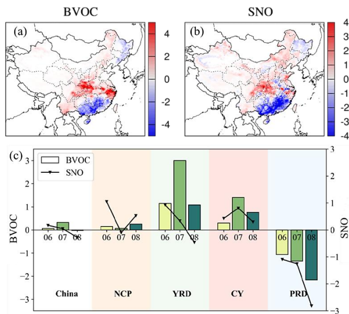
Figure 2. (a) The differences in simulated BVOC emission rates between BASE22 and BASE21 ( BASE22–BASE21 , units: mole s -1 ). (b) Same as (a) but for SNO (units: μmole s -1 ). (c) Differences of BVOC and SNO emission rates between summer 2022 and 2021 across different regions based on the MEGAN model.
