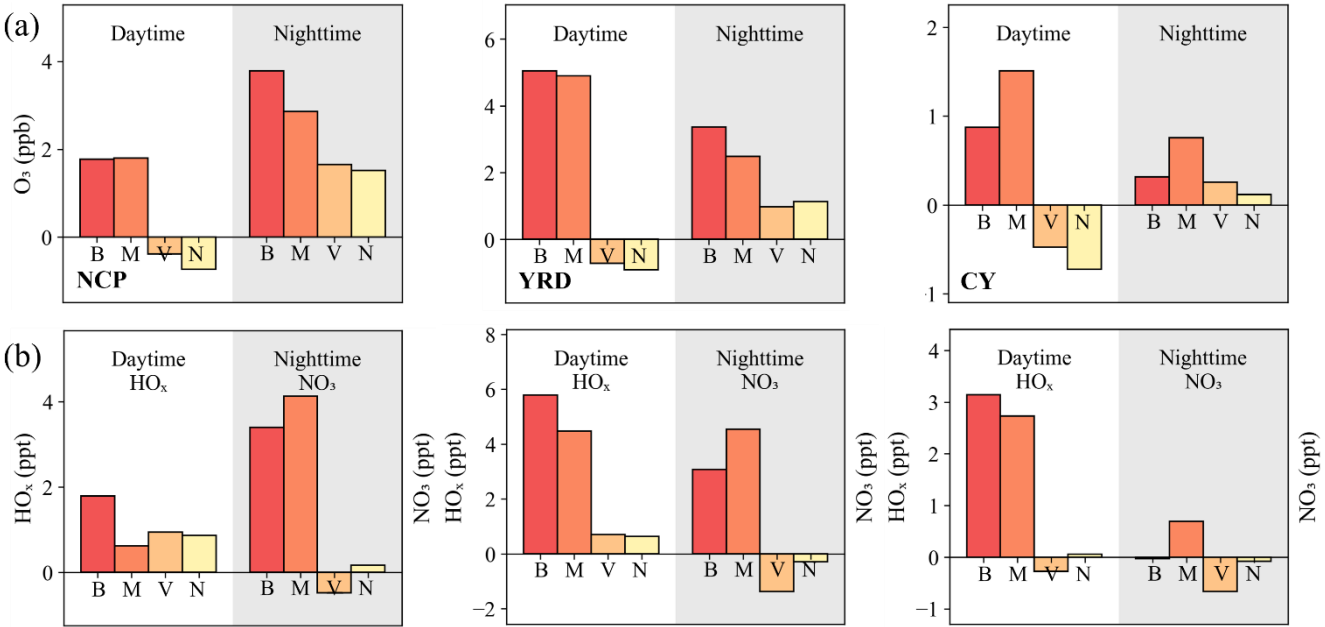
215 Figure 4. Diurnal differences in hourly (a) O 3 , (b) daytime HO x , and nighttime NO 3 concentrations in the NCP, YRD, and CY regions, respectively. Daytime is defined as 8:00 to 20:00 and nighttime as 20:00 to 8:00 Beijing Time (Zhu et al., 2020; Wang et al., 2022). The differences shown are BASE22–BASE21 (labelled ‘B’) for the total change between 2021 and 2022, BASE22–MET22 (labelled ‘M’) for the contribution of meteorology; BASE22–BVOC22 (labelled ‘V’) for weather-driven BVOC emission changes; and BASE22–SNO22 (labelled ‘N’) for weather-driven SNO emission changes.
