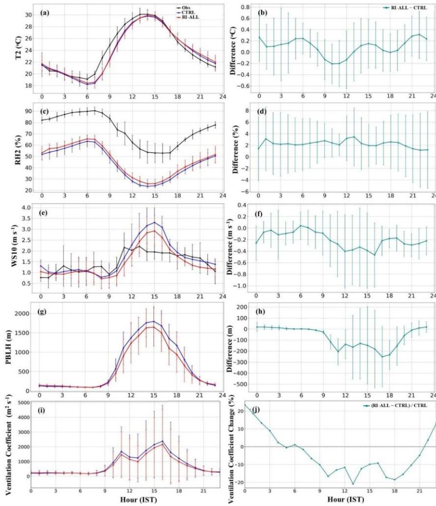
515 Fig. 5: Diurnal cycle of simulated meteorological parameters in CTRL and RI-ALLEXP5 along with observations, and changes in RI-ALLEXP5 with respect to CTRL averaged over Delhi for Event-I under clear-sky: (a) and (b) for T2, (c) and (d) for RH for RH2, (e) and (f) for WS10, and (g) and (h) for PBLH.
