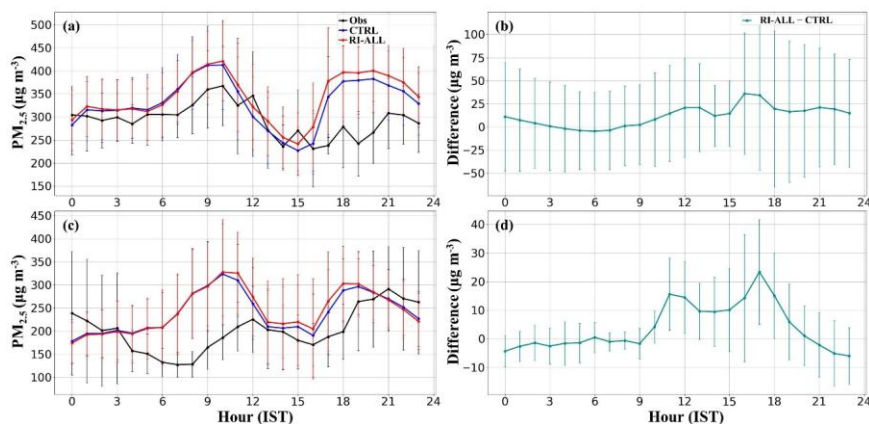
Fig. 7. Diurnal cycle of averaged simulated PM 2.5 mass concentrations in CTRL and RI-ALLEXP5 along with observations and changes in RI-ALLEXP5 with respect to CTRL: (a) and (b) for Event-I, and (c) and (d) for Event-II under clear-sky over Delhi .
