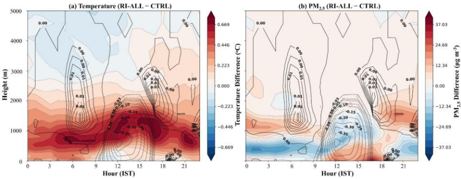
Fig. 6. Mean diurnal time–height cross-sections over Delhi showing the differences in (a) temperature (°C) and (b) PM 2.5 concentration (µg m -3 ) between the RI-ALL and CTRL simulations during Event-I. Filled contours represent the differences (RI-ALL – CTRL) in temperature and PM 2.5 concentration. Black contours denote differences in turbulent kinetic energy (TKE; m 2 s -2 ), with solid contours indicating positive differences and dashed contours indicating negative differences
