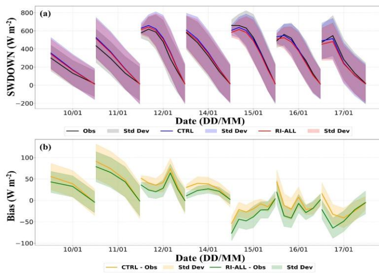
Fig. 3. (a) Time series of simulated SWDOWN in CTRL and RI-ALLEXP5 configuration along with observations over Delhi, and (b) bias in CTRL and RI-ALLEXP5 configurations during Event-II.
