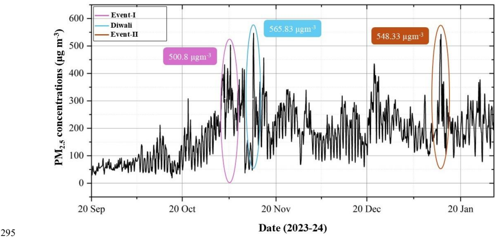
Fig. 1. Ground based PM 2.5 measurements over Delhi for the period between 20 September 2023 to 31 January 2024.
