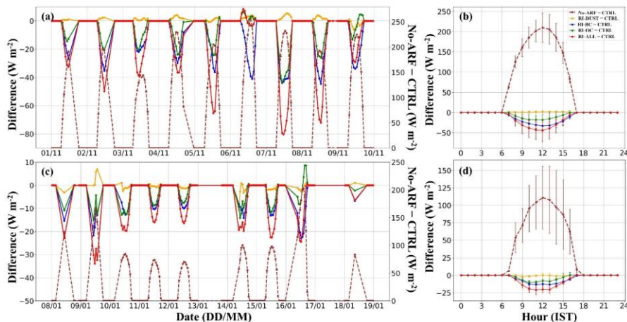
Fig. 4. Reduction in simulated SWDOWN in RI-DUSTEXP2 , RI-BCEXP3 , RI-OCEXP4 , and RI-ALLEXP5 configurations with respect to CTRL along with difference of No-ARFEXP4 configuration and CTRL during (a) Event-I, and (c) Event-II in clear-sky over Delhi . Diurnal changes in simulated averaged SWDOWN during (b) Event-I, and (d) Event-II in clear-sky over Delhi .
