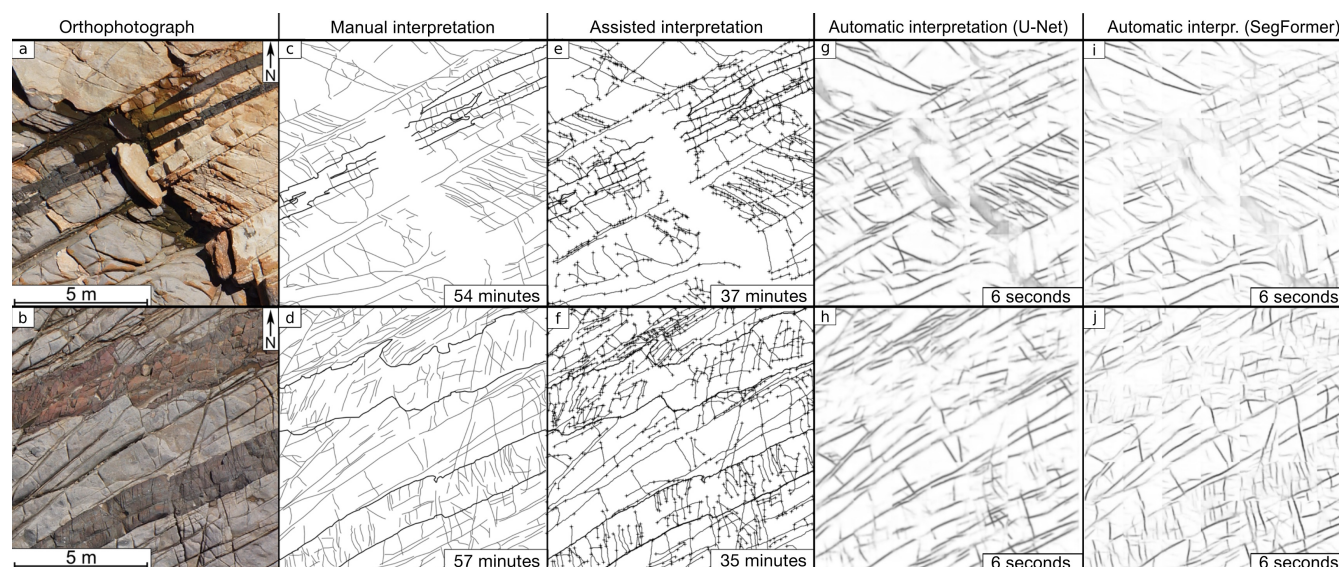
Figure 14. Two 10 \times 10 m orthophotographs (Thiele et al., 2017b) (a, b) with corresponding fracture traces digitised manually (Thiele et al., 2017b) (c, d), semi-automatically using the assisted method of (Thiele et al., 2017b) (e, f), automatically with the U-Net model (g, h) and with SegFormer model (i, j)
