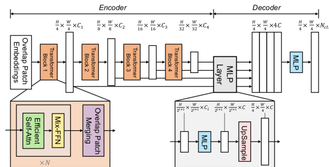
Figure 6. Overview of the SegFormer architecture combining a transformer encoder with a lightweight decoder (Xie et al., 2021)
