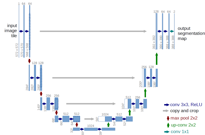
Figure 5. Overview of the U-Net encoder–decoder architecture with skip connections (Ronneberger et al., 2015)
