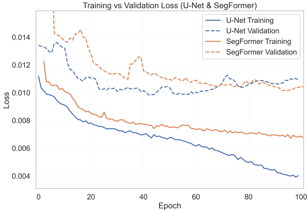
Figure 12. Training and validation loss curves for U-Net and SegFormer (range: [0, 1])
