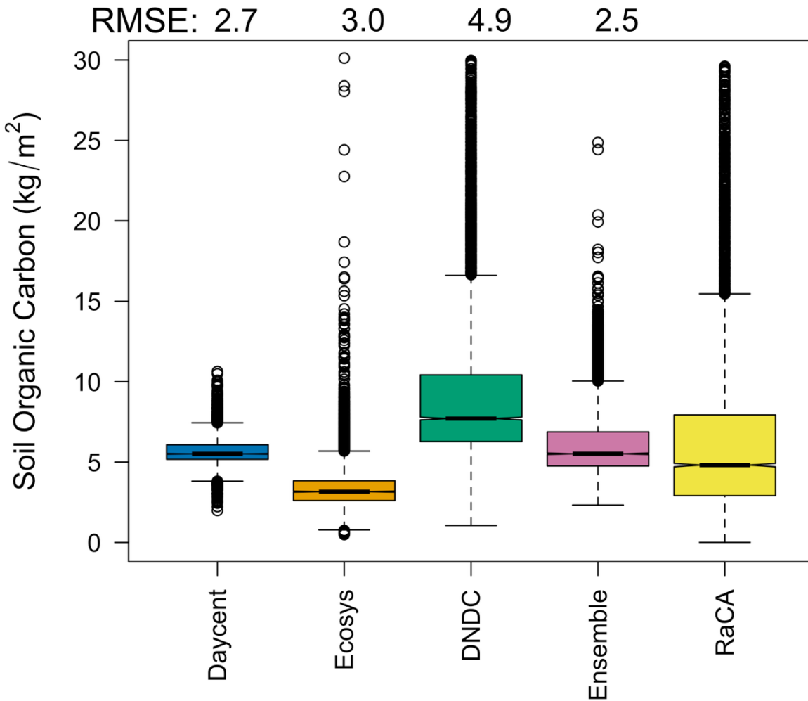
Figure 3 Comparison of observed soil organic carbon (SOC) stocks (0-30 cm) (kg C m 2 ) from the RaCA dataset with SOC simulated and root mean square error (kg C m 2 ) by individual agroecosystem models and the ensemble approach.
