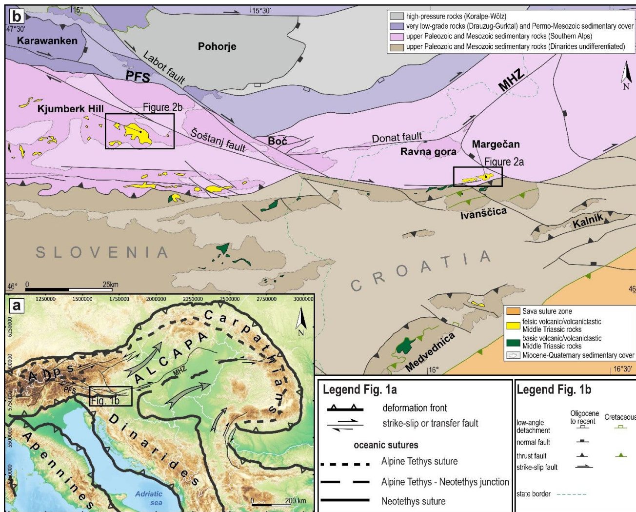
Figure 1 (a) Topographic map of the Alpine-Carpathian-Dinaridic orogen and Pannonian Basin region. Major tectonic boundaries after Schmid et al. (2020). (b) Tectonic map showing pre-Miocene tectonic units of the Dinarides and the Alps exposed from beneath the Neogene–Quaternary sedimentary cover (semi-transparent) after Schmid et al. (2020) and Fodor et al. (2021) modified according to Vukovski et al. (2024). PFS Periadriatic Fault System, MHZ Mid-Hungarian Shear Zone. Locations of Middle Triassic igneous and pyroclastic outcrops, outlines of Miocene to Quaternary sediments, locations and age of folds and faults are compiled after Tomljenović & Csonotos (2001), Fodor et al. (2021), Basic Geological Maps of former Yugoslavia on the 1:100,000 scale, sheets Klagenfurt (Buser and Cajhen, 1977), Kranj (Grad and Ferjančič, 1974), Ravne (Mioč et al., 1981), Ljubljana (Premru, 1982), Slovenj Gradec (Mioč and
