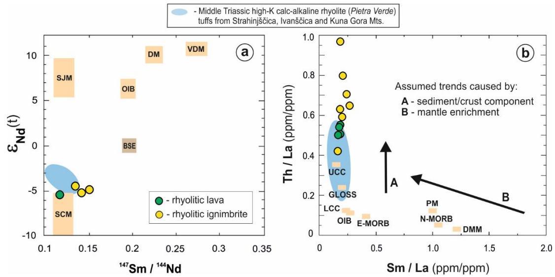
Figure 7 (a) ^{147}Sm/^{144}Nd - \epsilon_{Nd}(t) isotope ratios diagram for the rhyolitic lavas and rhyolitic ignimbrites from the Margečan area (N Croatia) and Kjumberk Hill (E Slovenia) [Hypothetical mantle sources: DM = depleted mantle (not refractory), VDM = very depleted mantle (refractory), SJM = subducted juvenile material (subducted oceanic crust; slab with little pelagic sediment), SCM = subducted continental material and BSE = bulk silicate earth. The observed compositions and hypothetical end members sources calculated for the Middle Triassic following Swinden et al. (1990)]. (b) Th/La – Sm/La diagram (after Plank, 2005) for the rhyolitic lavas (green dot) and rhyolitic ignimbrites (yellow dot) from the Margečan area (N Croatia) and Kjumberk Hill (E Slovenia). Abbreviations: [N-MORB = normal mid-ocean ridge basalts; E-MORB = enriched MORB; OIB = ocean island basalts; PM = primitive mantle (Sun and McDonough, 1989)]; [UCC = upper continental crust; LCC = lower continental crust (Rudnick and Gao, 2014)]; GLOSS = global subduction sediment (Plank and Langmuir, 1998); DMM = depleted MORB mantle (Workman and Hart, 2005). Middle Triassic high-K calc-alkaline rhyolitic tuffs from Strahinjčica, Ivanščica and Kuna Gora Mts. (Slovenec et al., 2023) are plotted for correlation constraints.
