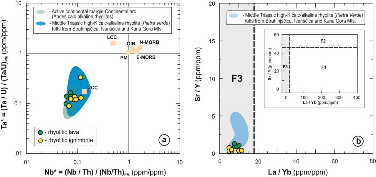
Figure 9 Discrimination diagrams for the rhyolitic lavas and rhyolitic ignimbrites from the Margečan area (N Croatia) and Kjumberski Hill (E Slovenia): (a) (Nb/Th)/(Nb/Th)_{PM} - (Ta/U)/(Ta/U)_{PM} plot (after Niu and Batiza, 1997; Niu et al., 1999). Abbreviations: [N-MORB = normal mid-ocean ridge basalts; E-MORB = normal mid-ocean ridge basalts; OIB = ocean island basalts; PM = primitive mantle (Sun and McDonough, 1989)]; [UCC = upper continental crust; LCC = lower continental crust (Rudnick and Gao, 2014)]. Data for Andes calc-alkaline rhyolites (Riley et al., 2001; Garrison et al., 2011) and Middle Triassic high-K calc-alkaline rhyolitic tuffs from Strahinjšica and Ivanščica Mts. (Slovenec et al., 2023) are plotted for correlation constrains. (b) La/Yb - Sr/Y plot (Halder et al., 2021 and references therein). Abbreviations: F1 = garnet stability field, little/no plagioclase, F2 = garnet and plagioclase stability field, F3 = plagioclase stability field, little/no garnet. Middle Triassic high-K calc-alkaline rhyolitic tuffs from Strahinjšica, Ivanščica and Kuna Gora Mts. (Slovenec et al., 2023) are plotted for correlation constrains.
