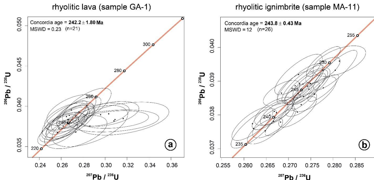
315 Figure 8 Concordia diagram and zircon U-Pb ages for the (a) Kjumbersk Hill rhyolitic lava and (b) Margečan rhyolitic ignimbrite. Discordant ages are not taken in to account.
