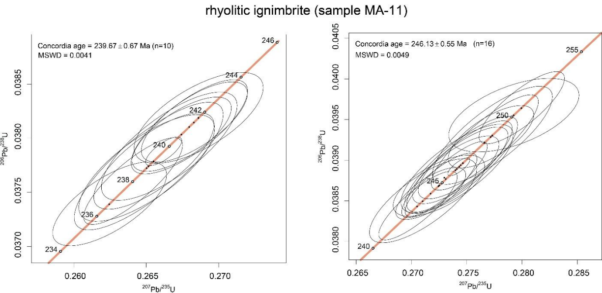
Figure H1 Concordia diagrams and zircon U-Pb ages for two possible zircon populations from the Margečan rhyolitic ignimbrite (sample MA-11). Discordant ages were not taken into account.
