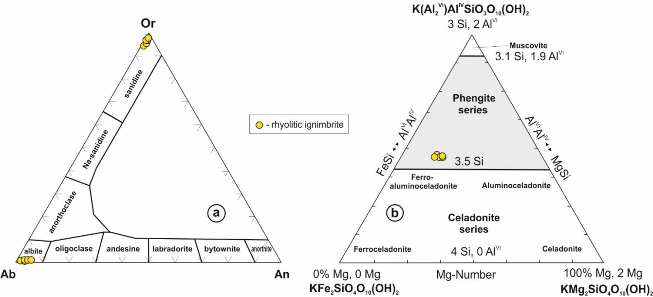
Figure 4 Classification diagrams for feldspar [Ab – An – Or plot; Deer et al., 1992; Dana et al., 1993] and mica [ K(Al_2^{VI})Al^{IV}SiO_3O_{10}(OH)_2 – KFe_2SiO_4O_{10}(OH)_2 – KMg_2SiO_4O_{10}(OH)_2 plot; taken from Tappert et al., 2013] from the rhyolitic ignimbrites from the Margečan area (N Croatia).
