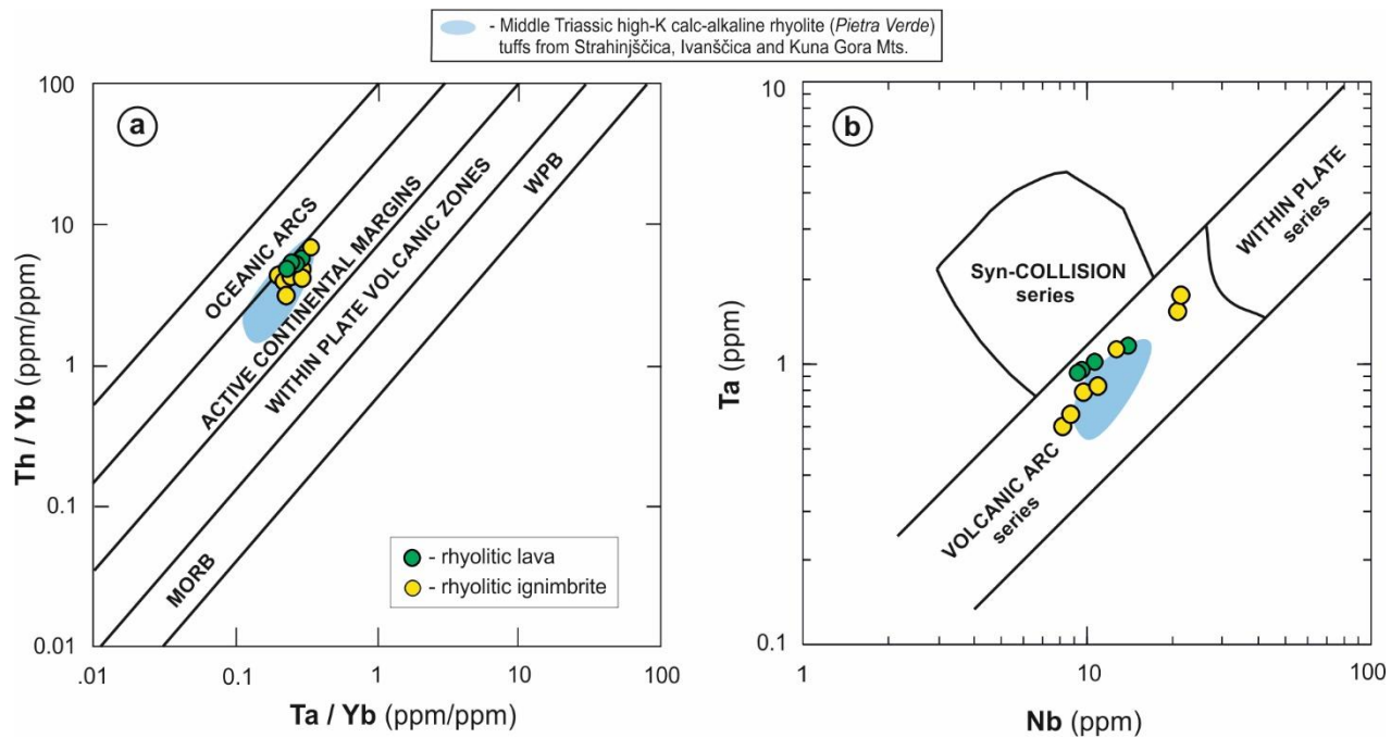
Figure 10 Discrimination diagrams for the rhyolitic lavas and rhyolitic ignimbrites from the Margečan area (N Croatia) and Kjumberk Hill (E Slovenia). (a) Ta/Yb – Th/Yb diagram (Gorton and Shandl, 2000). (b) Nb – Ta diagram (Pearce et al., 1984).
