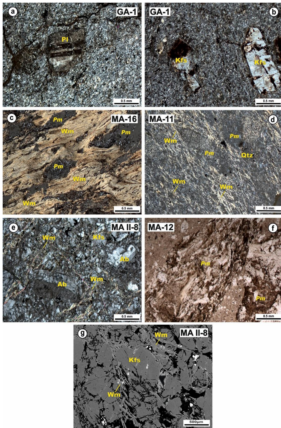
Figure 3 Micropetrographical characteristics of the Middle Triassic (a-b) rhyolitic lavas from the Kjumberski Hill (E Slovenia) and (c-f) rhyolitic ignimbrites from the Margečan area (N Croatia). (g) Back-scattered electron image of rhyolitic ignimbrite from Margečan locality
