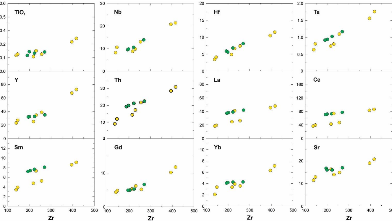
Figure E1 Variation diagrams for Zr as a differentiation index (e.g., Pearce, 1975) vs. TiO 2 and selected trace elements, as well as REE for the rhyolitic lavas (green dot) and rhyolitic ignimbrites (yellow dot) from the Margečan area (N Croatia) and Kjumberk Hill (E Slovenia).
