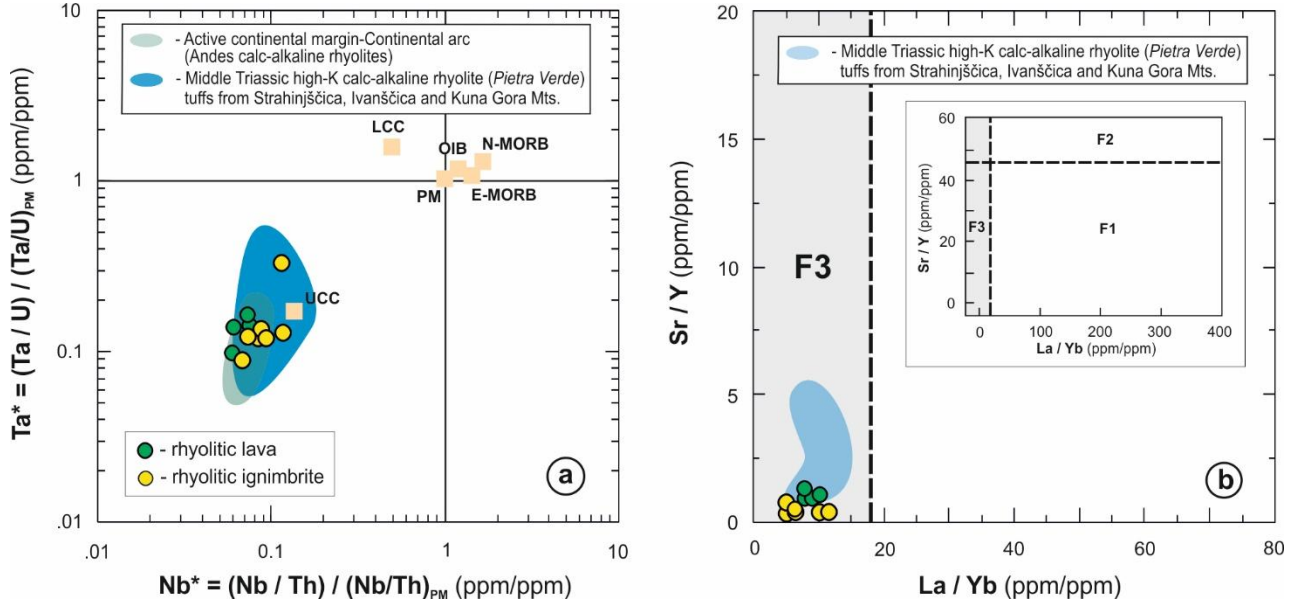
Figure 9 Discrimination diagrams for the rhyolitic lavas (green dot) and rhyolitic ignimbrites (yellow dot) from the Margečan area (N Croatia) and Kjumberski Hill (E Slovenia): (a) (Nb/Th)/(Nb/Th)_{PM} - (Ta/U)/(Ta/U)_{PM} plot (after Niu and Batiza, 1997; Niu et al., 1999). Abbreviations: [N-MORB = normal mid-ocean ridge basalts; E-MORB = normal mid-ocean ridge basalts; OIB = ocean island basalts; PM = primitive mantle (Sun and McDonough, 1989)]; [UCC = upper continental crust; LCC = lower continental crust (Rudnick and Gao, 2014)]. Data for Andes calc-alkaline rhyolites (Riley et al., 2001; Garrison et al., 2011) and Middle Triassic high-K calc-alkaline rhyolitic tuffs from Strahinjščica and Ivanščica Mts. (Slovenec et al., 2023) are plotted for correlation constrains. (b) La/Yb - Sr/Y plot (Halder et al., 2021 and references therein). Abbreviations: F1 = garnet stability field, little/no plagioclase, F2 = garnet and plagioclase stability field, F3 = plagioclase stability field, little/no garnet. Middle Triassic high-K calc-alkaline rhyolitic tuffs from Strahinjščica, Ivanščica and Kuna Gora Mts. (Slovenec et al., 2023) are plotted for correlation constrains.
