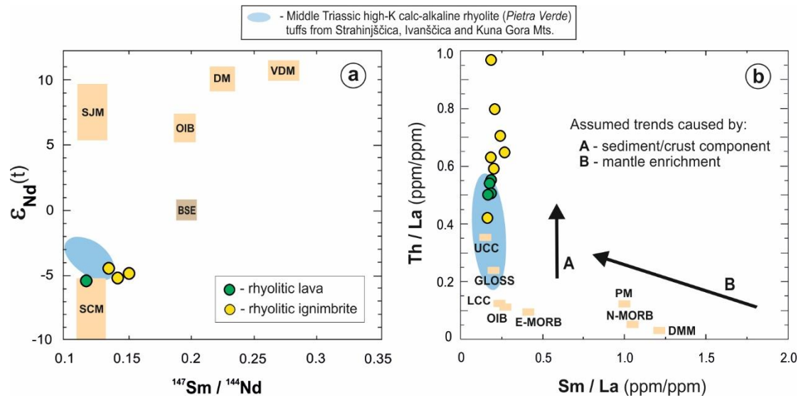
Figure 7 (a) ^{147}Sm / ^{144}Nd - \epsilon_{Nd}(t) isotope ratios diagram for the rhyolitic lavas (green dot) and rhyolitic ignimbrites (yellow dot) from the Margečan area (N Croatia) and Kjumberski Hill (E Slovenia) [Hypothetical mantle sources: DM = depleted mantle (not refractory), VDM = very depleted mantle (refractory), SJM = subducted juvenile material (subducted oceanic crust; slab with little pelagic sediment), SCM = subducted continental material and BSE = bulk silicate earth. The observed compositions and hypothetical end members sources calculated for the Middle Triassic following Swinden et al. (1990)]. (b) Th/La – Sm/La diagram (after Plank, 2005) for the rhyolitic lavas (green dot) and rhyolitic ignimbrites (yellow dot) from the Margečan area (N Croatia) and Kjumberski Hill (E Slovenia). Abbreviations: [N-MORB = normal mid-ocean ridge basalts; E-MORB = enriched MORB; OIB = ocean island basalts; PM = primitive mantle (Sun and McDonough, 1989)]; [UCC = upper continental crust; LCC = lower continental crust (Rudnick and Gao, 2014)]; GLOSS = global subduction sediment (Plank and Langmuir, 1998); DMM = depleted MORB mantle (Workman and Hart, 2005). Middle Triassic high-K calc-alkaline rhyolitic tuffs from Strahinjčica, Ivanščica and Kuna Gora Mts. (Slovenec et al., 2023) are plotted for correlation constraints.
