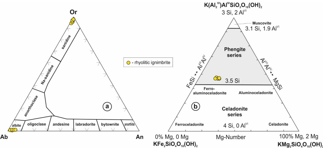
Figure 4 Classification diagrams for feldspar [Ab – An – Or plot; Deer et al., 1992; Dana et al., 1993] and mica [ K(Al_2^{VI})Al^{IV}Si_3O_{10}(OH)_2 – KFe_2Si_4O_{10}(OH)_2 – KMg_2Si_4O_{10}(OH)_2 plot; taken from Tappert et al., 2013] from the rhyolitic ignimbrites from the Margečan area (N Croatia).
