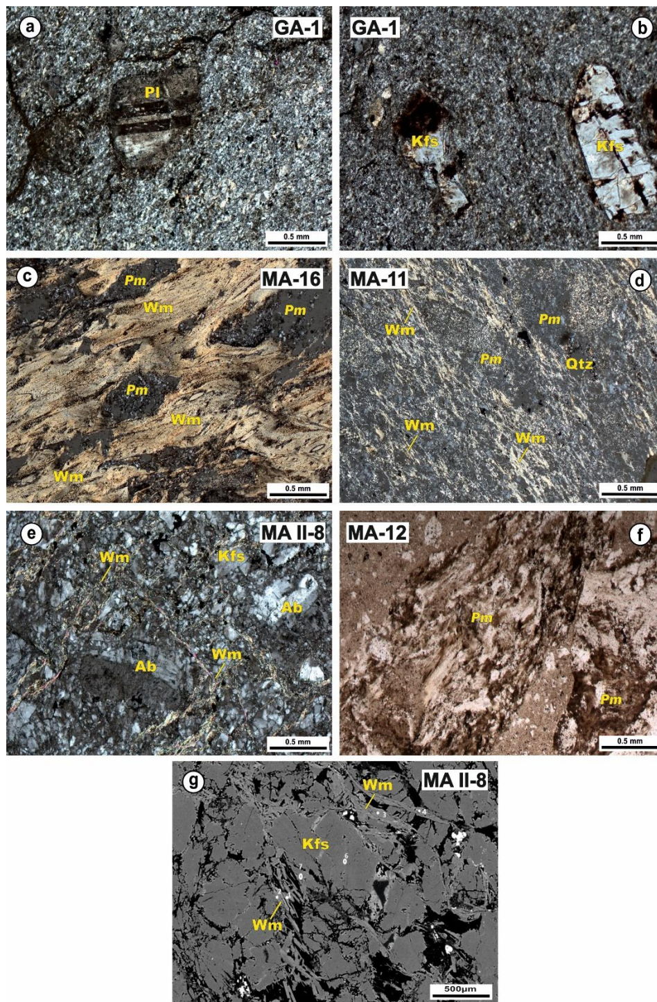
225 Figure 3 Micropetrographical characteristics of the Middle Triassic (a-b) rhyolitic lavas from the Kjumbersk Hill (E Slovenia) and (c-f) rhyolitic ignimbrites from the Margečan area (N Croatia). (g) Back-scattered electron image of rhyolitic ignimbrite from Margečan locality
