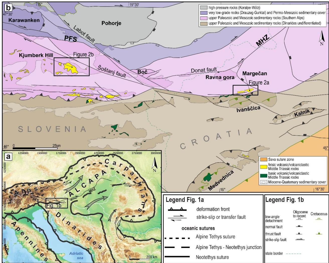
40 Figure 1 (a) Topographic map of the Alpine-Carpathian-Dinaridic orogen and Pannonian Basin region. Major tectonic boundaries after Schmid et al. (2020). (b) Tectonic map showing pre-Miocene tectonic units of the Dinarides and the Alps exposed from beneath the Neogene–Quaternary sedimentary cover (semi-transparent) after Schmid et al. (2020) and Fodor et al. (2021) modified according to Vukovski et al. (2024). PFS Periadriatic Fault System, MHZ Mid-Hungarian Shear Zone. Locations of Middle Triassic igneous and pyroclastic rocks outcrops , outlines of Miocene to Quaternary sediments, locations and age of folds and faults are compiled after Tomljenović & Csontos (2001), Fodor et al. (2021), Basic Geological Maps of former Yugoslavia on the 1:100,000 scale, sheets
