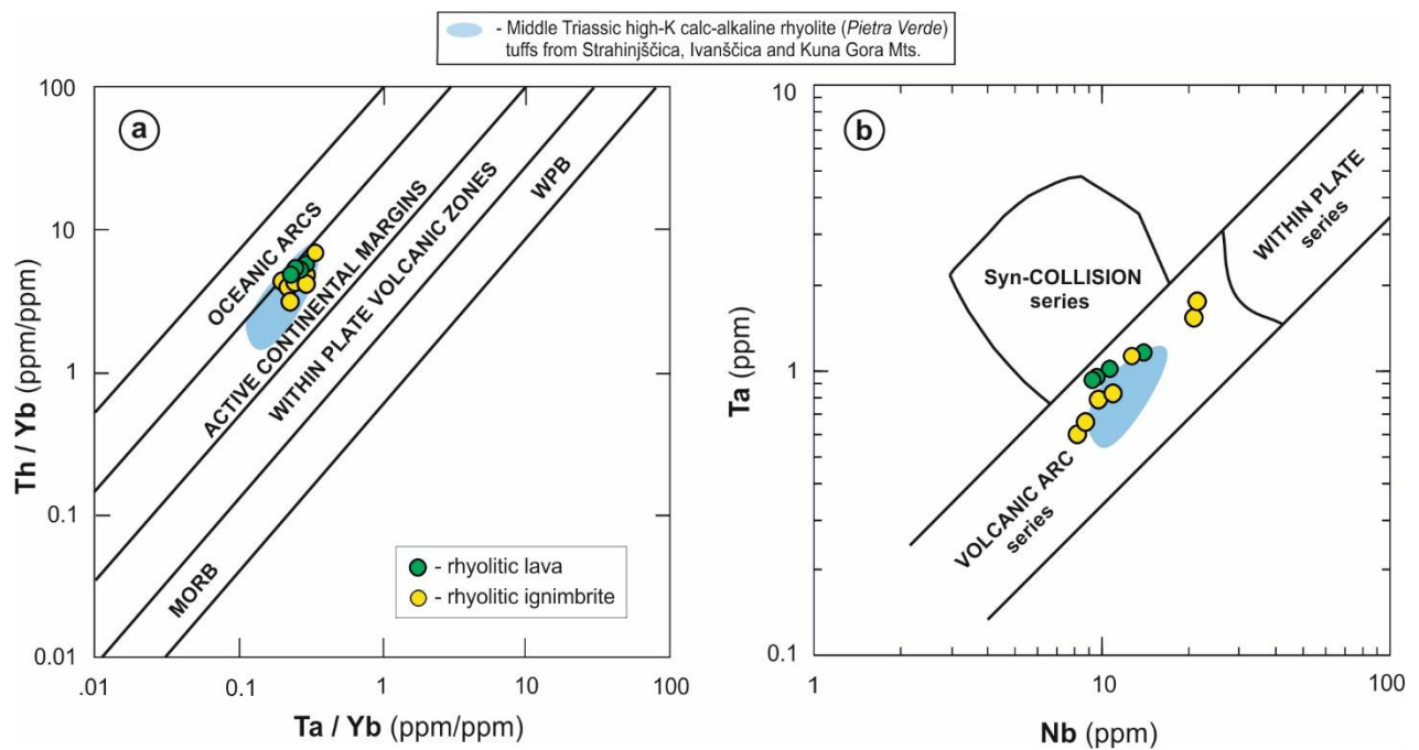
Figure 10 Discrimination diagrams for the rhyolitic lavas (green dot) and rhyolitic ignimbrites (yellow dot) from the Margečan area (N Croatia) and Kjumberski Hill (E Slovenia). (a) Ta/Yb – Th/Yb diagram (Gorton and Shandl, 2000). (b) Nb – Ta diagram (Pearce et al., 1984).
