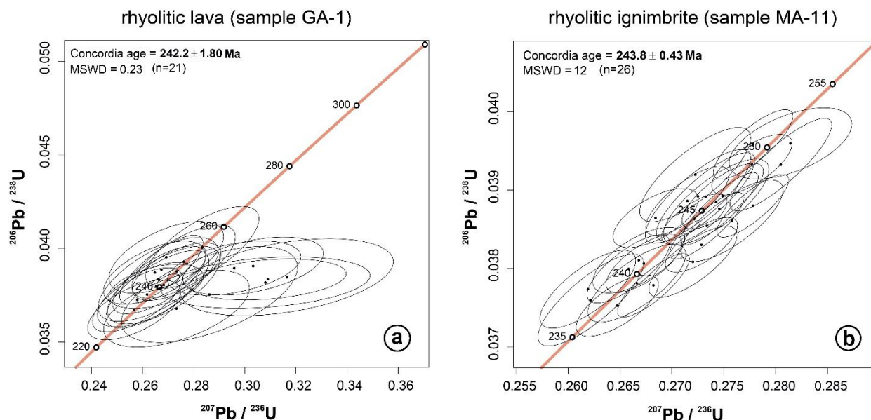
Figure 8 Concordia diagram and zircon U-Pb ages for the (a) Kjumberk Hill rhyolitic lava ( sample GA-1 ) and (b) Margečan rhyolitic ignimbrite ( sample MA-11 ). Discordant ages are not taken in to account.
