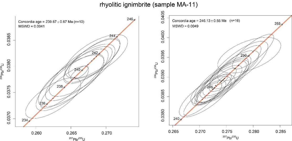
Figure H1 Concordia diagrams and zircon U-Pb ages for two possible zircon populations from the Margečan rhyolitic ignimbrite (sample MA-11). Discordant ages were not taken into account.
