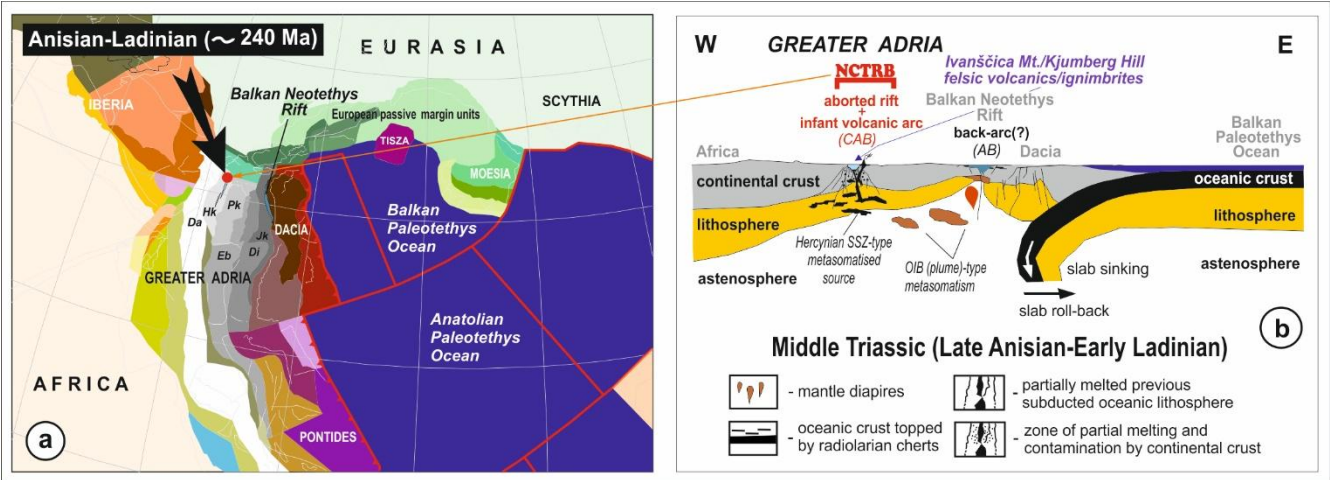
Figure 11 (a) The Anisian-Ladinian (~240 Ma) palaeogeographic reconstruction of the Mediterranean region simplified and slightly modified after van Hinsbergen et al. (2020) [Da = Dalmatian Nappe, Di = Drina-Ivanjica Nappe, Eb = East Bosnian-Durmitor Nappe, Jk = Jadar-Kopaonik Nappe, Hk = High-Karst Nappe, Pk = Pre-Karst Nappe] with location of investigated Margečan area (N Croatia) and Kjumberk Hill (E Slovenia) (marked with black arrow and red dot symbol). (b) Schematic geodynamic model (scale is approximate) for the central part of the Mediterranean region according to van Hinsbergen et al. (2020) palaeogeographic reconstruction shown in Fig. 11a. CAB = calc-alkaline and shoshonitic basalts/pyroclastites, AB = alkaline basalts, OIB = ocean island basalts; 1 = mantle diapires, 2 = oceanic crust topped by radiolarian cherts, 3 = partially melted previous subducted oceanic lithosphere, 4 = zone of partial melting and contamination by continental crust.
