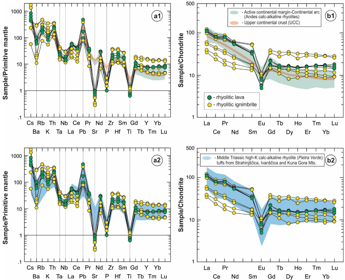
Figure 6 (a1, a2) Primitive mantle-normalised multielement and (b1, b2) REE patterns for the rhyolitic lavas (green-dot) and rhyolitic ignimbrites (yellow-dot) from the Margečan area (N Croatia) and Kjumberk Hill (E Slovenia). Normalisation values are from Sun and McDonough (1989) and Taylor and McLennan (1985). Pattern for upper continental crust (UCC; Rudnick and Gao, 2014), Andes calc-alkaline rhyolites (Riley et al., 2001; Garrison et al., 2011) and Middle Triassic high-K calc-alkaline rhyolitic tuffs from Strahinjščica, Ivanščica and Kuna Gora Mts. (Slovenec et al., 2023) are plotted for correlation constraints.
