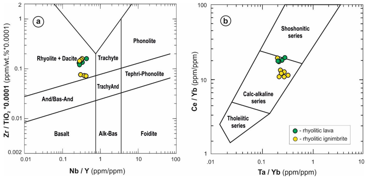
280 Figure 5 (a) Nb/Y – Zr/TiO 2 *10 -4 classification diagram (Pearce, 1996) and (b) Ce/Yb – Ta/Yb discrimination diagram after Pearce | (1982) for the rhyolitic lavas (green dot) and rhyolitic ignimbrites (yellow dot) from the Margečan area (N Croatia) and Kjumberk Hill (E | Slovenia).
