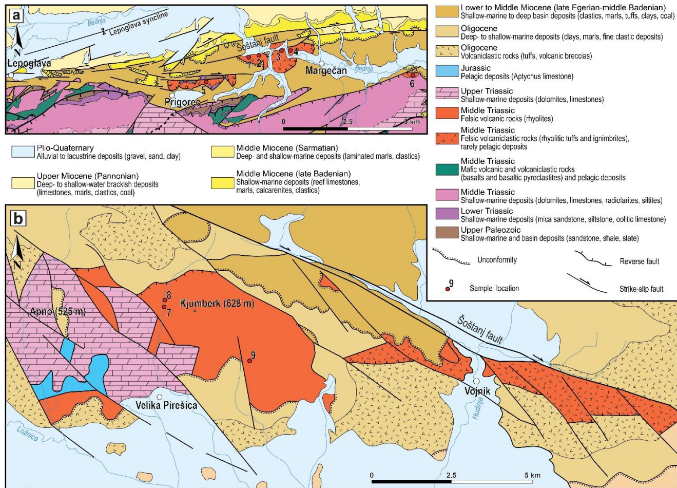
Figure 2 (a) Simplified geological sketch map of the northern Mt. Ivanščica and Margečan area in N Croatia (modified after Šimunić et al., 1982 and Vukovski et al., 2024). (b) Simplified geological sketch map of the wider Kjumberski Hill area in the eastern Slovenia (modified after Buser, 1977). Sample location: 1 = TSI-7, TSI-7A; 2 = MA-1, MA-2, MA-3, MA-4, MA-5, MA-6, MA-7, MA-8, MA-9,
