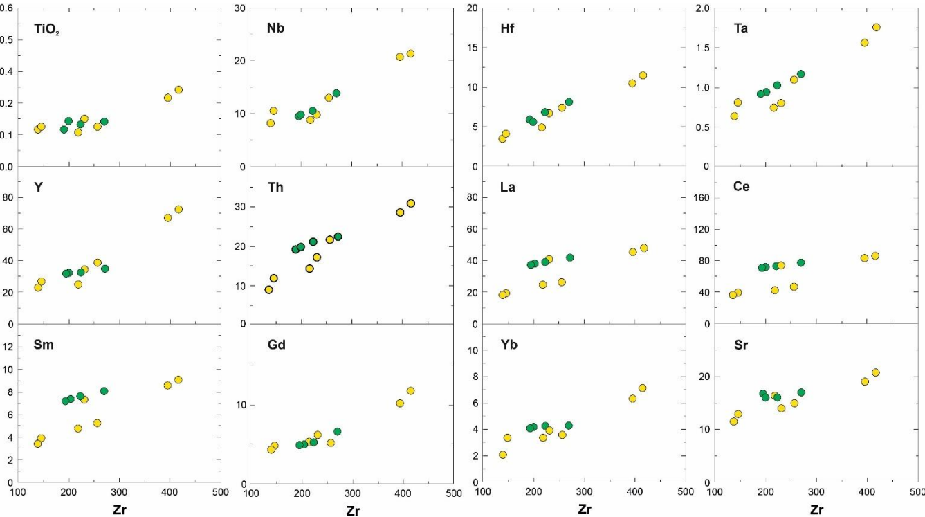
Figure G4-E1 Variation diagrams for Zr as a differentiation index (e.g., Pearce, 1975) vs. TiO 2 and selected trace elements and, as well as REE for the rhyolitic lavas (green dot) and rhyolitic ignimbrites (yellow dot) from the Margečan area (N Croatia) and Kjumberk Hill (E Slovenia).
