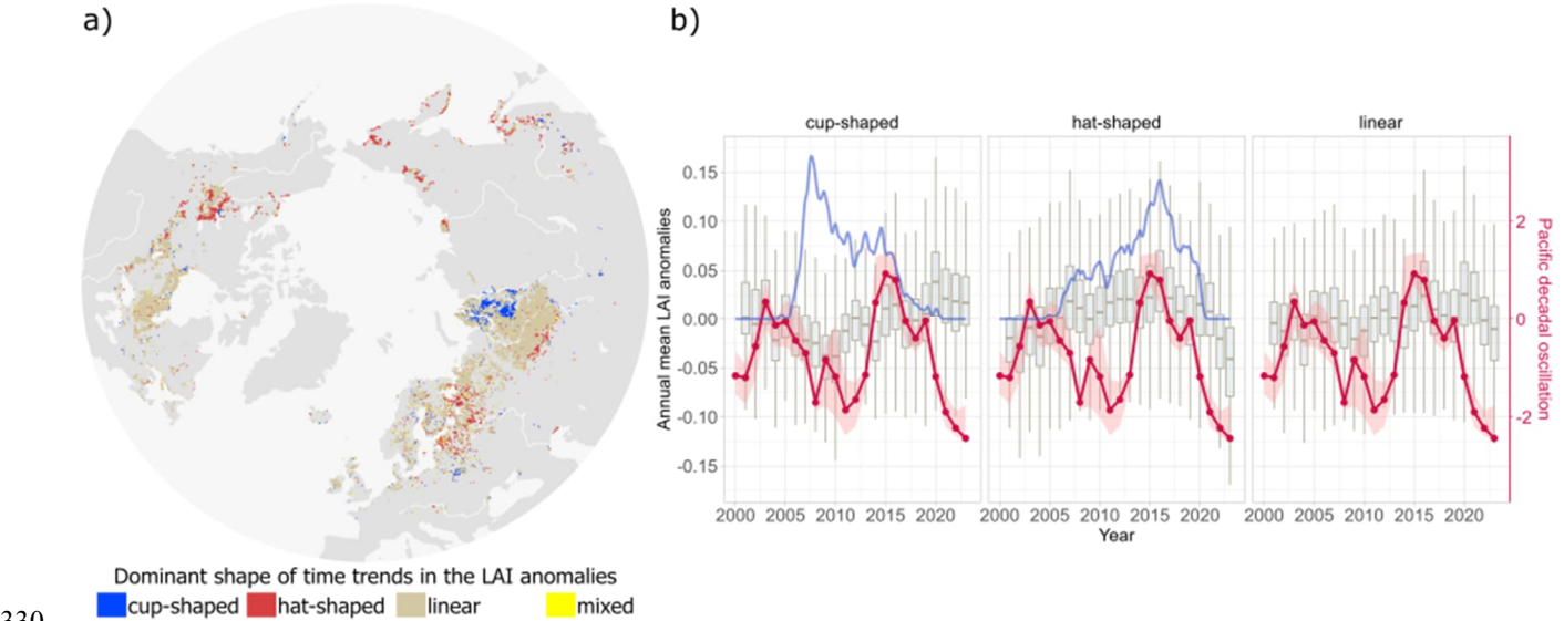
330 Figure 4: Spatial and temporal patterns of dominant LAI anomaly trends in northern peatlands. (a) Spatial distribution of the dominant trend shape in LAI anomalies, classified as cup-shaped, hat-shaped, linear, or mixed (where two or more shapes occurred with equal frequency within a hexagon). (b) Annual mean LAI anomalies (box plots) for pixels belonging to each trend type, overlaid with the density of posterior mean breakpoint years (blue line; higher values indicate more pixels with a breakpoint in that year) and the Pacific Decadal Oscillation (PDO) index (red line; shaded area shows 25–75% quantiles). 335
