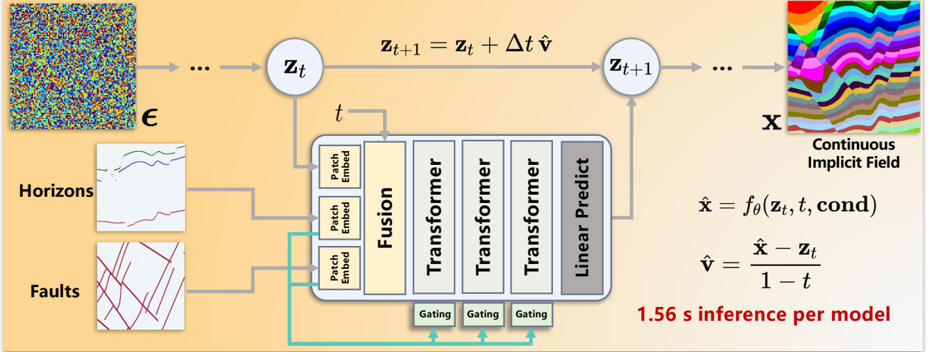
Figure 1. Overview of LFD for implicit structural modeling. Top: Training stage. We sample Gaussian noise \epsilon and time t , construct \mathbf{z}_t = t\mathbf{x} + (1-t)\epsilon , and use a structure-enhanced Transformer conditioned on horizons and faults to predict the clean implicit scalar field \hat{\mathbf{x}} . Bottom: Inference stage. Starting from \mathbf{z}_0 = \epsilon , we iteratively integrate the probability-flow ODE using \hat{\mathbf{x}} to obtain \hat{\mathbf{v}} and generate the final implicit structural model. Note that the implicit scalar field is a continuous-valued output, the colormap visualizations shown here use discrete color bins solely for display purposes.
