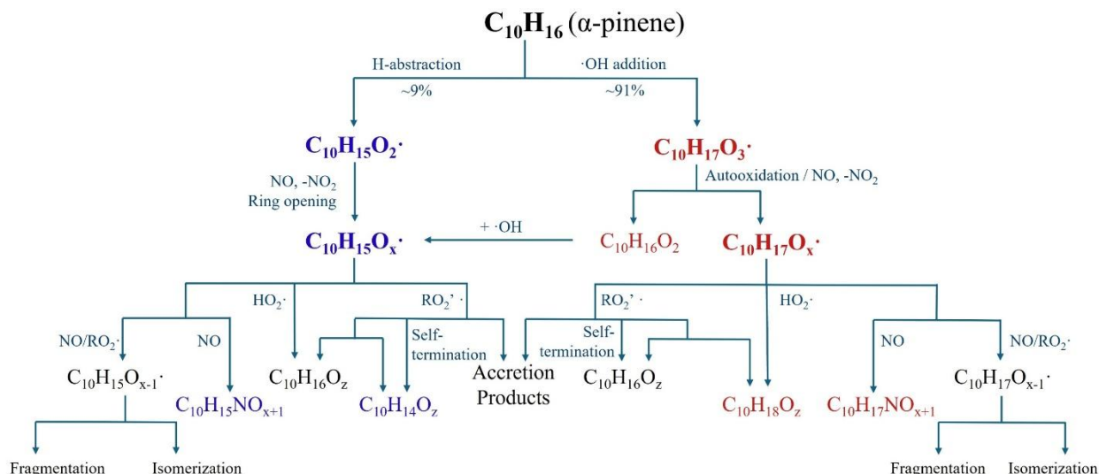
Figure 1. A schematic diagram illustrating \cdot OH initiated \alpha -pinene photooxidation through either the OH-addition pathway or the H-abstraction pathway. The unique peroxy radicals and their subsequent termination reactions are also depicted. The potential closure products are categorized into different families based on their formation pathways and the number of hydrogen atoms in molecules.
