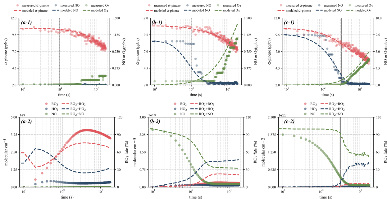
240 Figure 2. Results of model simulations for \alpha -pinene photooxidation under NO-free (a-1, a-2), low-NO (b-1, b-2), and high-NO conditions (c-1, c-2). The upper panels show modelled and measured concentrations of \alpha -pinene, NO, and \text{O}_3 across the three conditions, while the lower panels show the corresponding radical concentrations of \text{RO}_2\cdot and \text{HO}_2\cdot . In addition, the lower panels illustrate the relative contributions of \text{RO}_2\cdot + \text{HO}_2\cdot , \text{RO}_2\cdot + \text{RO}_2\cdot and \text{RO}_2\cdot + \text{NO} reactions to the total bimolecular reaction rate of \text{RO}_2\cdot (shown as \text{RO}_2\cdot fate on the right y-axis).
