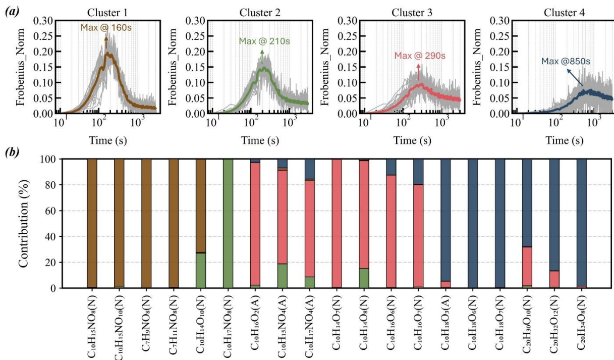
Figure 4. Results of fuzzy c-means clustering for the dominant peaks (156 in total) during early reaction stages of \alpha -pinene photooxidation under high NO condition are shown in panel (a). The four-cluster solution is shown here. The time series of the cluster centers are displayed as colored solid lines, while individual species are shown in gray lines. Panel (b) illustrates the cluster apportionment of selected major products detected in both nitrated-CIMS (N) and amine-CIMS (A).
