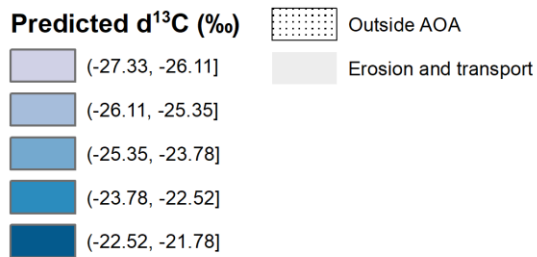
Figure 8. Stable carbon isotope ( \delta^{13}\text{C} ) values. Predictions outside the area of applicability (AOA) of the model are shown as well.
