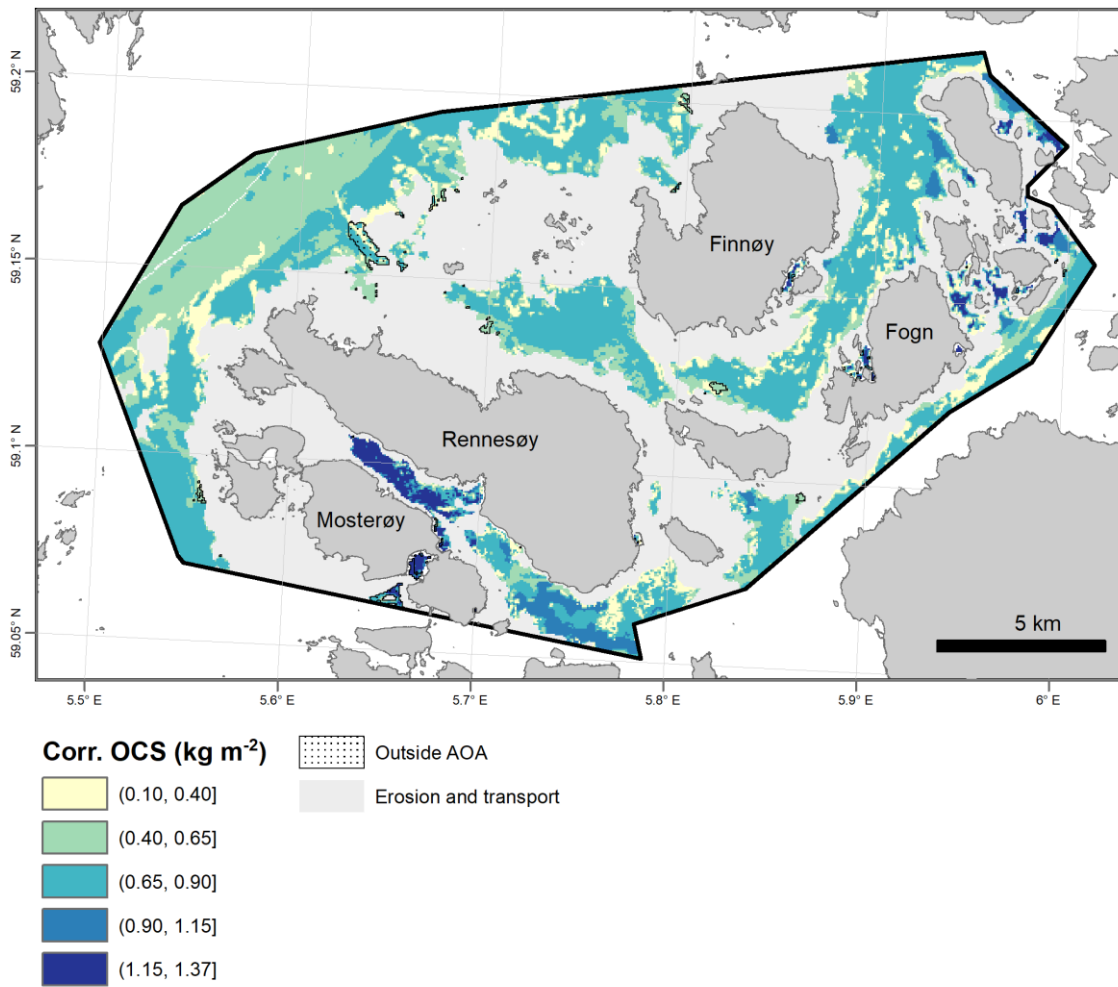
Figure 7. Corrected organic carbon stocks (OCS) of the upper 10 cm of the sediment. Predictions outside the area of applicability (AOA) of the model are shown as well.
