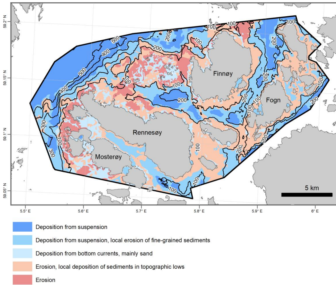
775 Figure 4. Sedimentary environment in the core study site. Isobaths are shown in 100 m-intervals.
