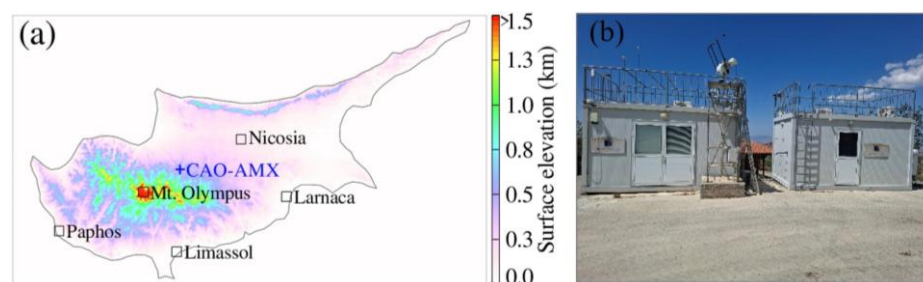
120 Figure 1: (a) Surface elevation map of Cyprus, showing the location of the CAO-AMX measurement station (blue marker) in the foothills of the Troodos Mountains. Major cities (Paphos, Limassol, Larnaca, and Nicosia) and Mount Olympus (the highest point in Cyprus) are indicated by open square boxes. Elevation data are taken from the U.S. Geological Survey global digital elevation model (DEM) with a horizontal resolution of 30 arc seconds (approximately 1 km; GTOPO30). (b) Image of the CAO-AMX station, consisting of two containers housing 125 advanced instrumentation for condensing vapours, trace gases, and aerosols.
