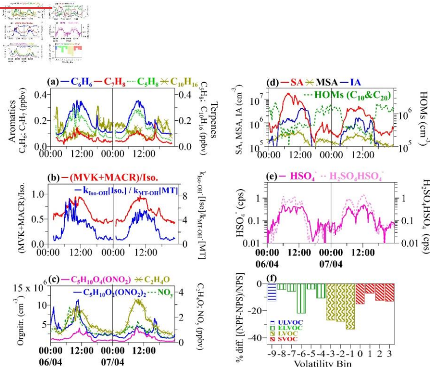
Figure S7: Median diurnal variation of aerosol precursors and condensing vapours during the consecutive NPF-NPS events observed during 6-7 April. (a) mixing ratios of benzene ( C_6H_6 ), toluene ( C_7H_8 ), isoprene ( C_5H_8 ), and monoterpenes ( C_{10}H_{16} ); (b) the ratio of the sum of methyl vinyl ketone (MVK) and maethacrolein (MACR) to the isoprene [(MVK+MACR)/Iso.] and the relative OH reaction rates of isoprene and MTs ( k_{Iso-OH}[Iso.]/k_{MT-OH}[MT] ); (c) organonitrates [ C_5H_{10}O_4(ONO_2) and C_5H_{10}O_2(ONO_2)_2 ], acetaldehyde ( C_2H_4O ) and reactive nitrogen compounds ( NO_y ); (d) concentrations of sulfuric acid (SA), methyl sulfonic acid (MSA), iodic acid (IA), and highly oxygenated organic molecules (HOMs, C_{10} & C_{20} ); (e) ambient ion mode signals of bisulfate monomer ( HSO_4^- ) and dimer ( H_2SO_4HSO_4^- ) in counts per second (cps); (f) percentage difference in organic vapour concentrations (molecules cm^{-3} ) between the NPF and NPS events as a function of volatility bin, expressed as \log_{10} of the effective saturation concentration, \log_{10}(C^*) . Negative percentage differences indicate higher organic vapour concentrations during the NPS event. ULVOC, ELVOC, LVOC, and SVOC denote ultra-low volatile organic carbon, extremely low volatile organic carbon, low volatile organic carbon, and semi-volatile organic carbon, respectively.
