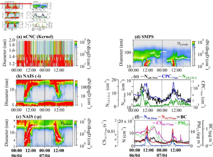
Figure 3: Median diurnal variation of aerosol properties during the consecutive NPF (6 April) and NPS (7 April) events. Particle size distributions measured by (a) nCNC, (b-c) NAIS negative polarity ions and particles, and (d) SMPS. Concentrations of (e) negative polarity ions in the 2.0-2.3 nm size range measured by NAIS ( N_{2.0-2.3(-i)} ), sub-3nm particles measured by nCNC ( N_{sub-3nm} ), and >7nm particles measured by CPC ( N_{>7nm} ); (f) nucleation mode ( N_{10-25nm} ) and total particle ( N_{10-777nm} ) number concentrations from SMPS, total condensation sink ( CS_{10-777nm} ), and particulate matter of aerodynamic diameter less than 2.5 \mu m ( PM_{2.5} ) and black carbon (BC) mass concentrations.
