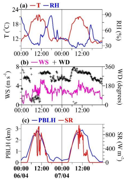
Figure 4: Median diurnal variation of meteorological parameters during the consecutive NPF-NPS events (6-7 April). (a) air temperature (T) and relative humidity (RH), (b) wind speed (WS) and wind direction (WD), and (c) planetary boundary layer height (PBLH) and solar radiation (SR).
