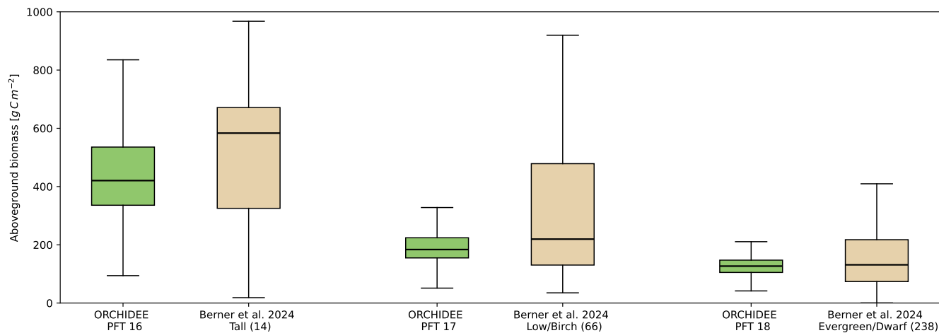
Figure 3. Simulated (green, ORCHIDEE-18, 1992-2020) and observed (light brown, Berner et al. (2024)) aboveground biomass for three shrub PFTs across the Arctic and Boreal Arctic-Boreal region. Observed biomass from Berner et al. (2024) was filtered to match the ORCHIDEE shrub PFT classification. Numbers in parentheses indicate the number of field sites included after filtering. Boxplots show median (center line), interquartile range (boxes) and whiskers extend to the farthest data point lying within 1.5x the interquartile range. A complete visualisation including outliers is shown in Fig. B1.
