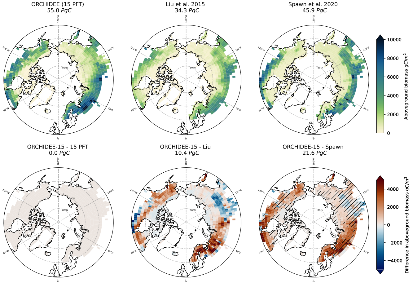
Figure B4. Simulated (ORCHIDEE with 15 PFTs) and observation-based (from Spawn et al. (2020) and Liu et al. (2015)) panarctic pan-Arctic AGB in 2010. Difference maps between ORCHIDEE with 15 PFTs and the observation-based products. Hatching indicates agreement with Spawn et al. (2020) standard error interval. Numbers indicate total AGB across the region (top row), and total difference (bottom row).
