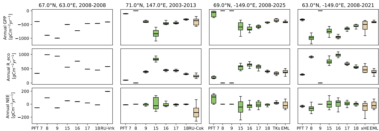
Figure B3. Simulated (green) and observed (brown) annual sum of CO_2 fluxes at three shrub-tundra four ORCHIDEE grid cells and six EC sites ( columns as in Figure 4 ). Rows represent CO_2 fluxes: gross primary productivity (GPP), ecosystem respiration ( R_{eco} ), and net ecosystem exchange (NEE). Negative values indicate uptake of CO_2 from the atmosphere by the vegetation, while positive values denote release.
