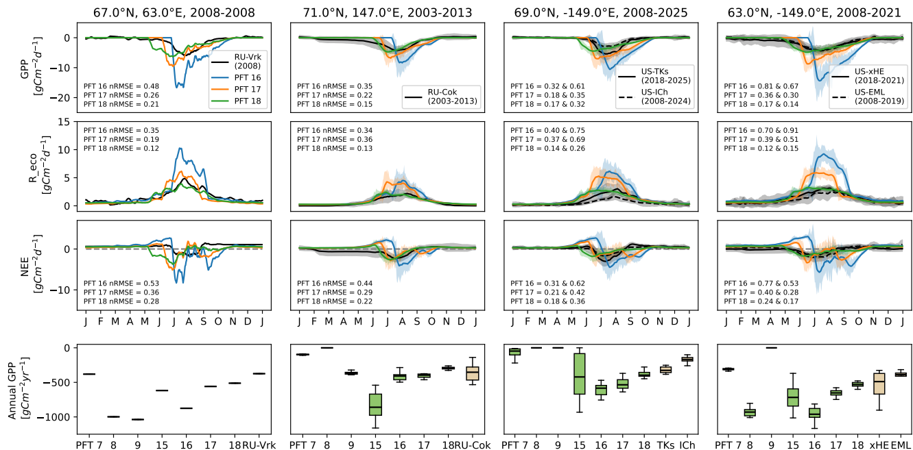
Figure 4. Simulated-Observed (color)-and-observed (black) CO_2 fluxes at three-six shrub-tundra EC sites and simulated (color) shrub CO_2 fluxes at four ORCHIDEE grid cells (columns, where the coordinates above the figures represent the centre of the 2^\circ \times 2^\circ grid cells). Rows represent CO_2 fluxes: gross primary productivity (GPP), ecosystem respiration ( R_{eco} ), and net ecosystem exchange (NEE). Negative values indicate uptake of CO_2 from the atmosphere by the vegetation, while positive values denote release. Shown is the average seasonal cycle and standard deviation (shading) in daily resolution, smoothed with a 10-day running mean. Goodness of fit is measured with root mean square error normalised by amplitude (nRMSE). Last row: annual sum of GPP simulated for all high-latitude PFTs in ORCHIDEE (green) and observed at the EC sites (brown). Note that where two EC sites are located in one ORCHIDEE grid cell, the observed fluxes shown represent different time frames and the ORCHIDEE fluxes are shown for the combined time frame.
