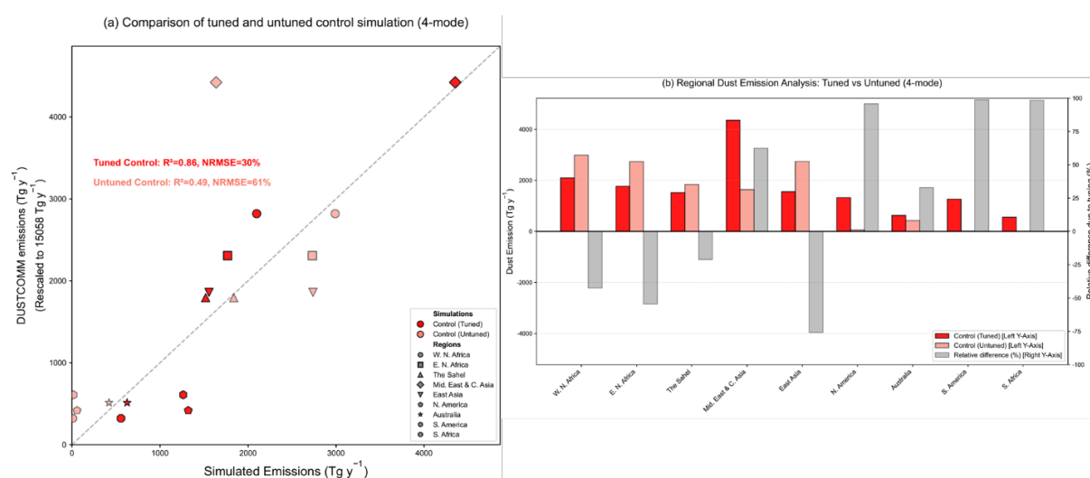
Figure S16. Comparison of tuned and untuned dust emission in the control simulation (4-mode configuration). (a) Regional evaluation of simulated dust emissions against DustCOMM constraints (Kok et al., 2021b) without (untuned; pink markers) and with (tuned; red markers) regional rescaling. The DustCOMM emissions were rescaled to the global total of the tuned control simulation for direct comparison. The 1:1 line (dashed), R^2 , and NRMSE are provided for reference. (b) Regional dust emission magnitudes in tuned (red bars) and untuned (pink bars) control simulations (left Y-axis), and the corresponding relative difference due to tuning (grey bars; right Y-axis). The relative difference is calculated as (tuned–untuned)/tuned.
