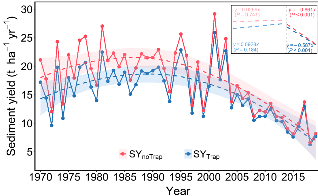
Figure 7. Interannual variations in average sediment yield (SY) with ( SY_{\text{Trap}} ) and without ( SY_{\text{noTrap}} ) sediment trapping by check dams during 1970–2020 in the middle Yellow River Basin. The dashed line represents a fitted curve, with the shaded area indicating the 95% confidence interval. The inset in the upper right displays the linear regression trend of SY before and after 2001.
