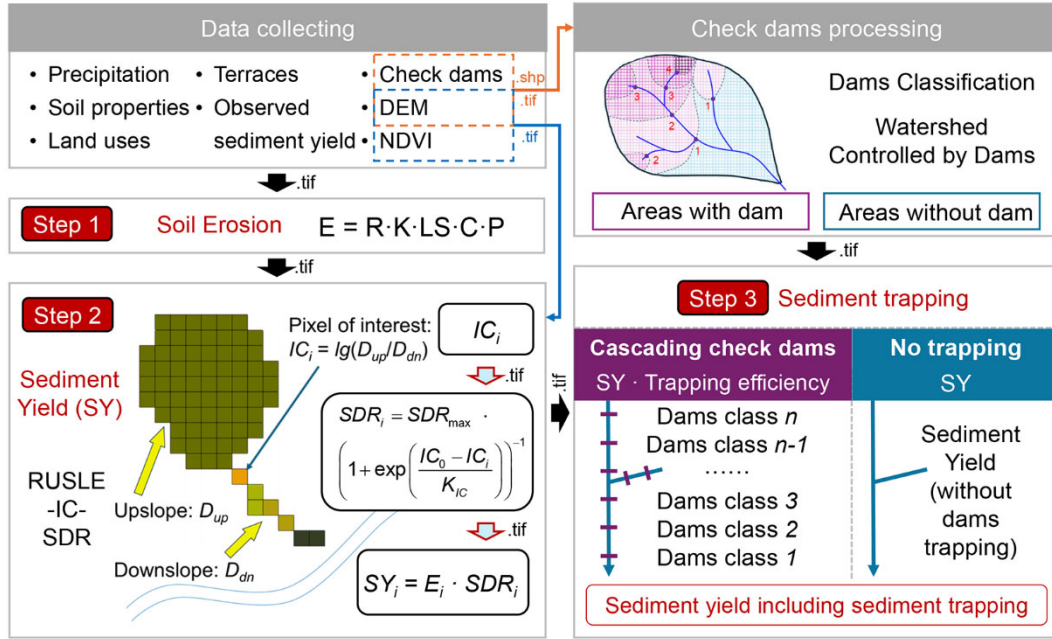
Figure 2. Framework of the integrated model for simulating sediment yield in the basin with cascading check dams. Step 1 denotes the soil erosion module by RUSLE . Step 2 indicates the sediment yield module by “ RUSLE-IC-SDR ” method. Step 3 represents the sediment trapping module by check dam. IC represents the index of connectivity, and SDR denotes the sediment delivery ratio.
