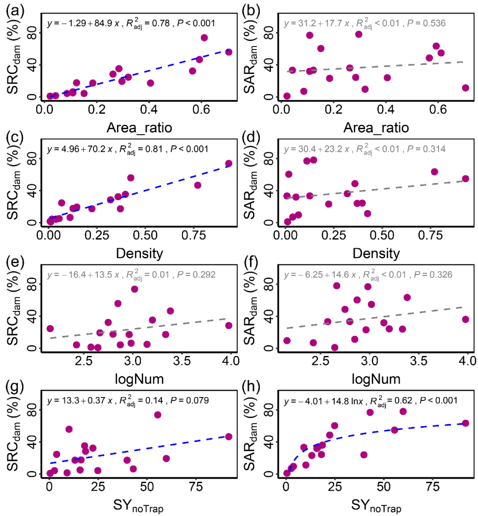
Figure 10. Correlations of sediment-Sediment reduction-Reduction contribution-Contribution of check dams (SRC dam ) and proportion of accumulated sediment relative to total storage capacity (SAR dam ) with the proportion of area controlled by check dams to the total basin area (Area_ratio) (a and b), check dam density (Density) (c and d), logarithm of the number of check dams (logNum) (e and f), and average sediment yield without sediment trapping by check dams (SY noTrap ) in sub-basins (g and h).
