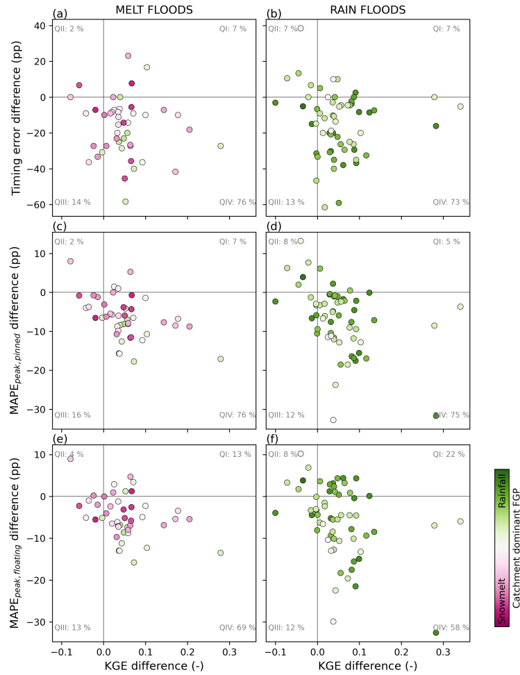
Figure C9. Model difference (i.e. LSTM minus HBV) in the overall performance metric KGE (x-axis) versus the flood peak metrics: (a–b) timing error, (c–d) MAPE_{peak, pinned} and (e–f) MAPE_{peak, floating} , separately for snowmelt generated floods (left) and rainfall generated floods (right). Each dot represents a catchment and is coloured by the catchment’s dominant flood generating process (FGP; ref. Fig. 2). Catchments within quadrant IV (QIV; lower right square) have a better score for LSTM as compared to HBV both in terms of overall performance score (KGE) and flood peak performance score. Percentages of catchments within each quadrant are given in the corners of the plots.
