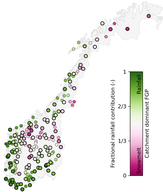
Figure 2. Average fractional rainfall (i.e. proportion of total) contribution to all observed flood events in the period 1994–2023 01.09.1994–31.08.2024 , and its relation to the catchment dominant flood generating process (FGP). Dark pink (green) dots represent catchments with snowmelt (rainfall) as their dominant FGP, whereas near-white dots represent catchments with similar average contributions from rainfall and snowmelt. All 200 catchments used for training the LSTM are shown, with thicker circles representing the 103 catchments used for model evaluation.
