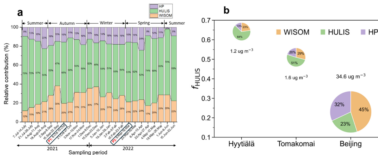
640 Figure 13 (a) Relative contributions of HP-WSOM, HULIS, and WISOM to total OAs. (b) Annual mean values of the proportions of HP-WSOM, HULIS, and WISOM with annual average OA concentrations at three sites in Hyttiälä, Tomakomai, and Beijing.
