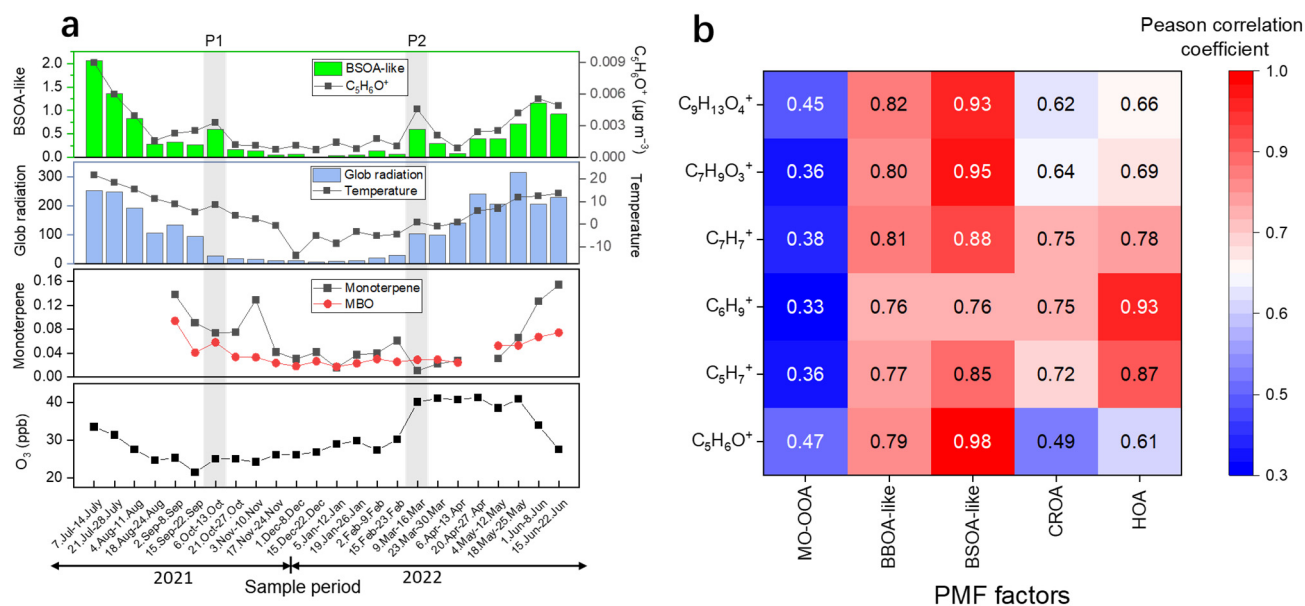
430 Figure 5 (a) Time series of BSOA-like factor and C_5H_6O^+ concentration, along with those of global radiation, temperature, monoterpenes, MBO, and O_3 (data from SmartSMEAR: https://smear.avaa.csc.fi/ ). (b) Correlation matrix illustrating the relationships between PMF-derived factors and the sum of characteristic fragment ions from HP-WSOM, HULIS, and WISOM.
