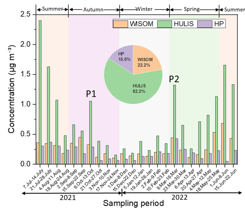
310 Figure 2 Seasonal variations in HP-WSOM, HULIS, and WISOM measured by HR-AMS, with the fractional contributions of their averages shown in the pie chart.
