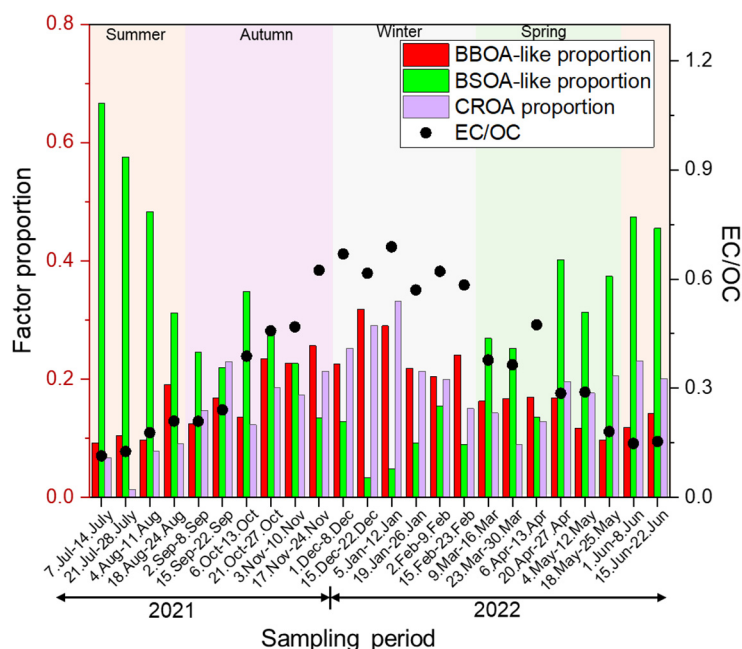
520 Figure 9. Seasonal variations in the relative contributions of BBOA-like, BSOA-like, and CROA factors, together with the EC/OC ratio.
