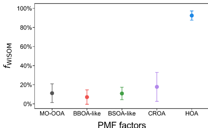
Figure 12. Proportions of the water-insoluble fractions of the five PMF factors. The markers and bars represent the mean and standard deviation, respectively.
