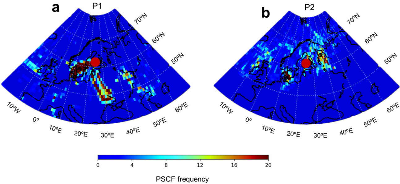
Figure 3 Potential source contribution function (PSCF) maps based on the 75th percentile of the DMPS-derived particle volume concentrations in the 100–1000 nm range. (a) P1 (October 6–13, 2021). (b) P2 (March 9–16, 2022).
