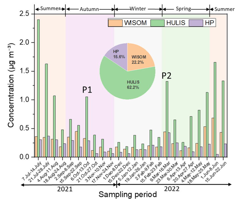
310 Figure 2 Seasonal variations in HP-WSOM, HULIS, and WSOM measured by HR-AMS, with the fractional contributions of their averages shown in the pie chart.
