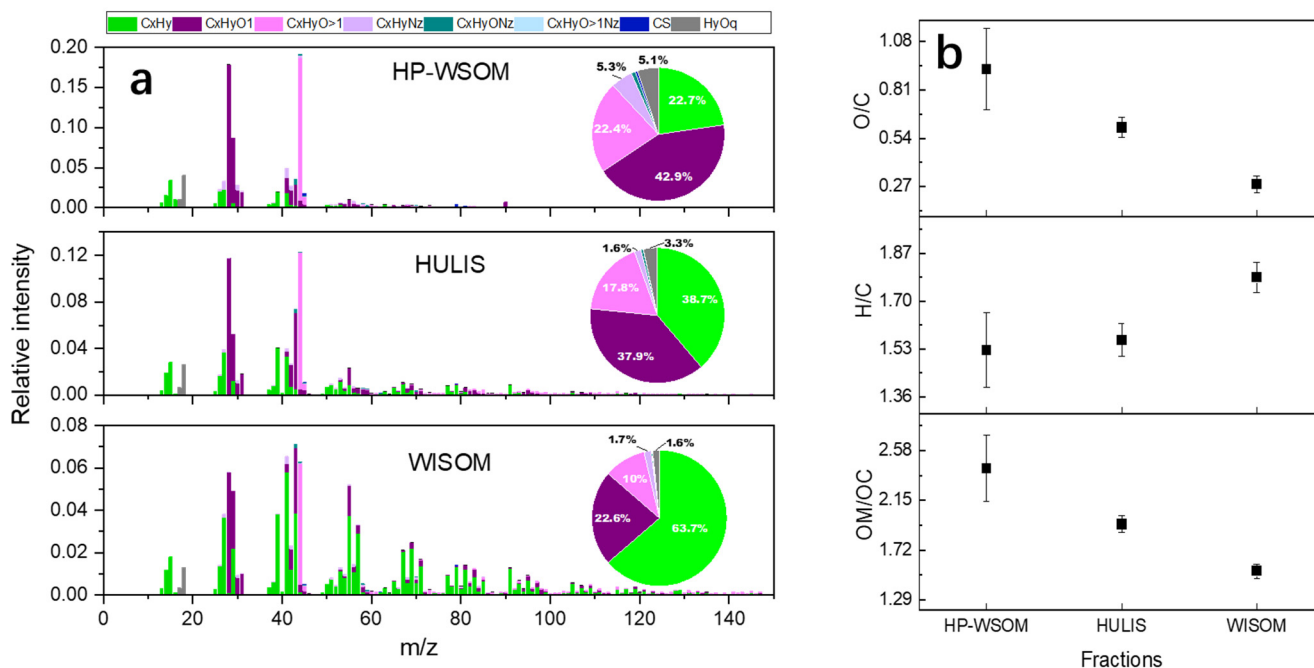
Figure 1(a) Averages of the normalized HR-AMS spectra for HP-WSOM, HULIS, and WISOM with pie charts showing the averages of the fractional contributions of fragment ion groups. Different fragment groups are represented by different colors in the stacked bars. (b) O/C and H/C ratios and OM/OC mass ratios of HP-WSOM, HULIS, and WISOM.
