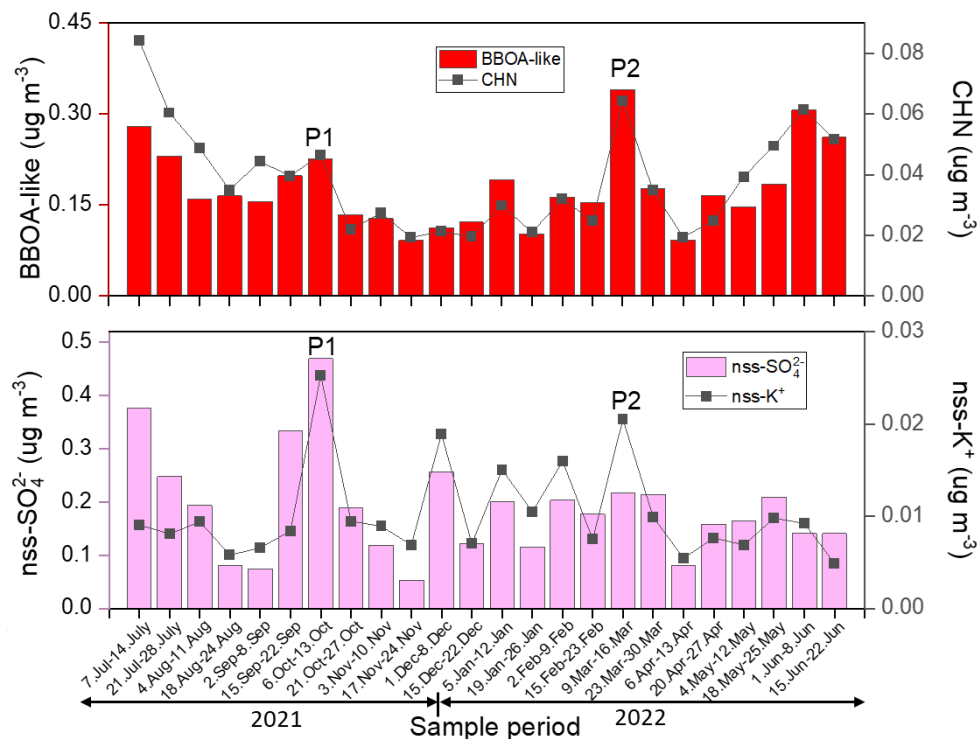
Figure 7. Time series of BBOA-like factor, CHN family ions, \text{nss-SO}_4^{2-} and \text{nss-K}^+ .
