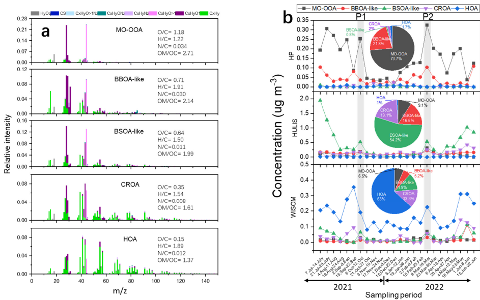
Figure 4. (a) HR-AMS spectra of the five PMF-derived factors and their elemental analysis data. (b) Time series of the concentrations
