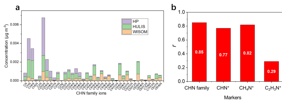
Figure 8 (a) Annual average concentrations of the OA mass detected as different CHN family ions in HP-WSOM, HULIS, and WISOM. (b) Correlation coefficients of the time series of BBOA-like factor with the series of total CHN family ions and individual ions ( \text{CHN}^+ , \text{CH}_4\text{N}^+ , and \text{C}_2\text{H}_3\text{N}^+ ).
