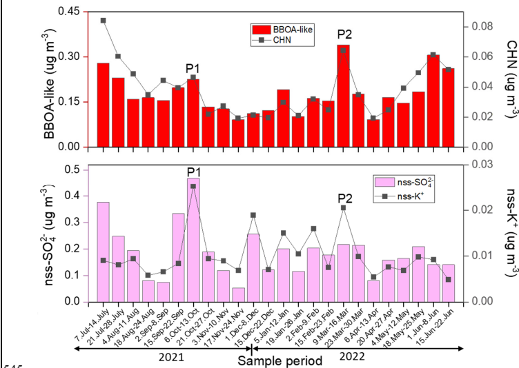
Figure 7. Time series of BBOA-like factor, CHN family ions, \text{nss-SO}_4^{2-} and \text{nss-K}^+ .
