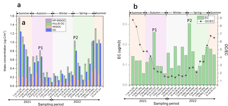
Figure S2. (a) Seasonal variations in the carbon concentrations of the HP-WISOM, HULIS, and WISOM fractions (HP-WISOC, HULIS-OC, and WISOC, respectively), and the concentrations of OC from the thermal/optical carbon analysis.. (b) The variations in the concentrations of EC and the OC/EC ratios.
