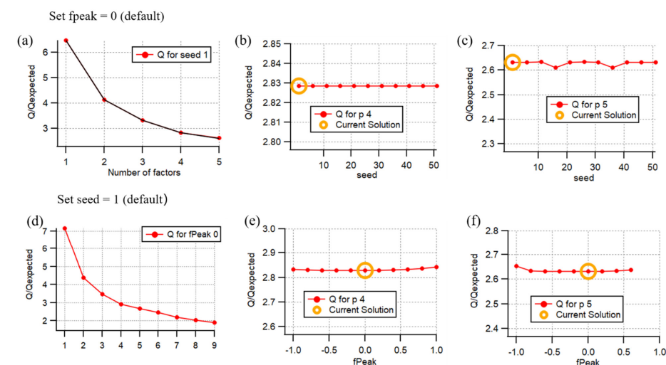
Figure S4. Evaluation of the PMF solutions using Q/Q_{\text{expected}} as a function of the number of factors, seed values, and fPeak values: (a) Q/Q_{\text{expected}} as a function of the number of factors for seed = 1; (b) Q/Q_{\text{expected}} as a function of seed for the 4-factor solution; (c) Q/Q_{\text{expected}} as a function of seed for the 5-factor solution; (d) Q/Q_{\text{expected}} as a function of the number of factors for fPeak = 0; (e) Q/Q_{\text{expected}} as a function of fPeak for the 4-factor solution; (f) Q/Q_{\text{expected}} as a function of fPeak for the 5-factor solution.
