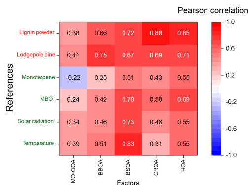
520 Figure 6. Pearson correlation coefficients between PMF-resolved OA factors and six selected references. The references include two meteorological parameters (temperature and solar radiation, data from SmartSMEAR) and two BVOCs (monoterpene and MBO, also from SmartSMEAR), for which correlations are based on temporal variations, as well as two biomass burning HR-AMS spectra for which correlations are based on mass spectral similarity (from the AMS Spectral Database, URL: http://cires.colorado.edu/jimenez-group/AMSsd/ ) (Ulbrich et al., 2009b).
