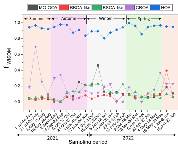
Figure 12. Seasonal variations in the water-insoluble fraction of the five PMF factors.
