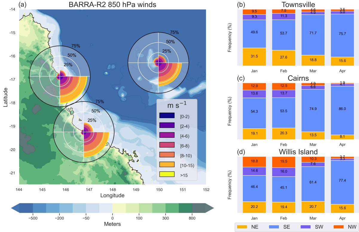
Figure 3. (a) Polar histograms over the CBS for BARRA-R2 850 hPa wind regimes defined in Section 2.2. Bar length indicates wind direction frequency, with colours indicating corresponding wind speeds in \text{m s}^{-1} . (b,c,d) shows the monthly regime frequency for Townsville, Cairns and Willis Island. BARRA-R2 850 hPa winds are averaged over each site’s radar domain (see Fig. 1) for the CBS over the period 1979–2024.
