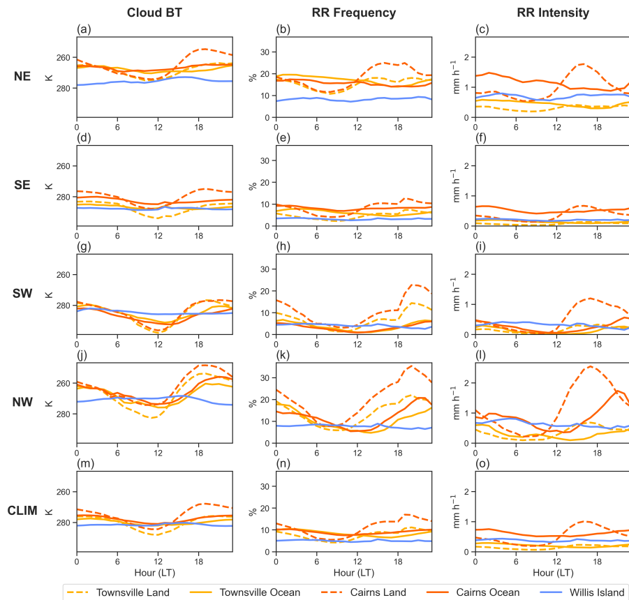
Figure 6. Diurnal cycle of Himawari–8 satellite channel 13 BT ( 10.4\ \mu\text{m} infrared wavelength band), radar retrieved rainfall frequency (percentage of points greater than 0.001\ \text{mm h}^{-1} ) and intensity (mean rain rate) calculated over the CBS for each wind regime and site. Each row shows the corresponding BT, rainfall frequency and rainfall intensity with consistent y-axes for each wind regime– with different colored lines for each site. Townsville and Cairns are separated into land (dashed) and ocean (solid) domains, associated with their radar coverage. The BT y-axis is inverted, so that peaks in the diurnal cycle indicate colder BTs. Rain intensity is calculated for all periods of valid data (not just raining periods).
