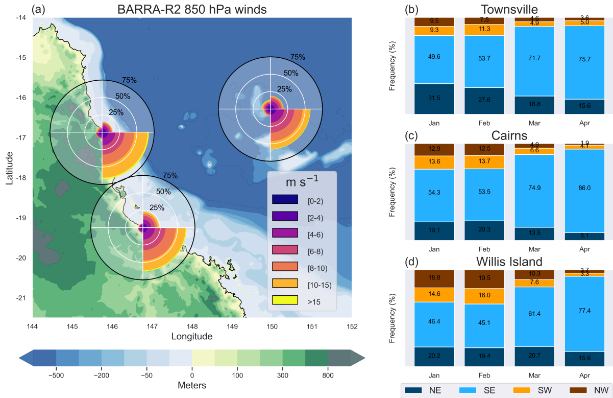
Figure 3. (a) Polar histograms over the CBS for BARRA–R2 850 hPa wind regimes defined in Section 2.2. Bar length indicates wind direction frequency, with and colours indicating indicate the corresponding wind speeds in \text{m s}^{-1} . (b,c,d) shows the monthly regime frequency for Townsville, Cairns and Willis Island. BARRA–R2 850 hPa winds are averaged over each site’s radar domain (see Fig. 1) for the CBS over the period 1979–2024.
