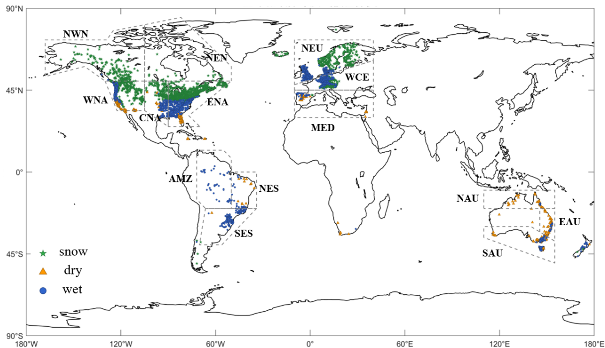
255 256 Figure 2. Spatial distribution of 6603 sample catchments for analysis. Green stars, orange triangles, and blue circles indicate the 257 catchments in snow, dry, and wet climate zones, respectively. AMZ, Amazon; CNA, central North America; EAU, eastern Australia; ENA, 258 eastern North America; MED, Mediterranean; NAU, northern Australia; NEN, north-eastern North America; NEU, northern Europe; NES, 259 northeastern South America; NWN, northwestern North America; SAU, southern Australia; SES, southeastern South America; WCE, 260 western and central Europe; WNA, western North America.
