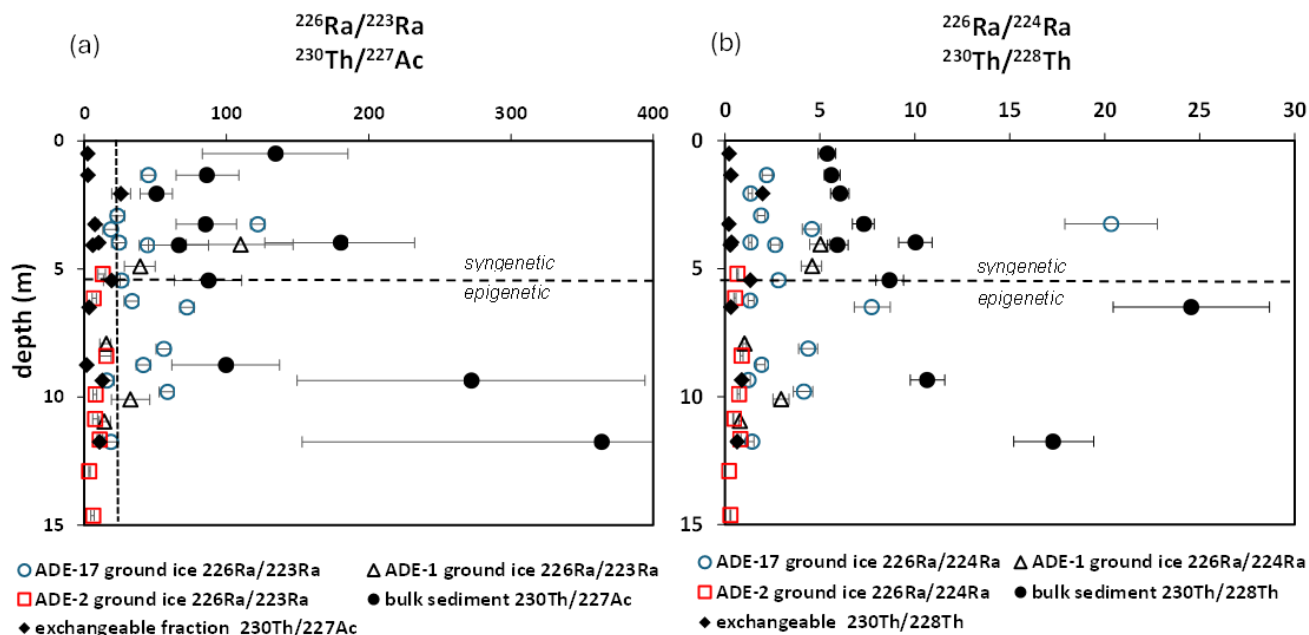
Figure 8: Radium isotope activities in ground ice and their parent ratios in bulk soil grains and on grain surfaces (exchangeable fraction). (a) (^{226}\text{Ra}/^{223}\text{Ra})_{\text{AR}} and (^{230}\text{Th}/^{227}\text{Ac})_{\text{AR}} ; (b) (^{226}\text{Ra}/^{224}\text{Ra})_{\text{AR}} and (^{230}\text{Th}/^{228}\text{Th})_{\text{AR}} . The vertical dotted line in (a) indicates the natural ratio of (^{238}\text{U}/^{235}\text{U}) , parents of ^{226}\text{Ra} and ^{223}\text{Ra} , respectively. The dashed line as in Figure 3.
