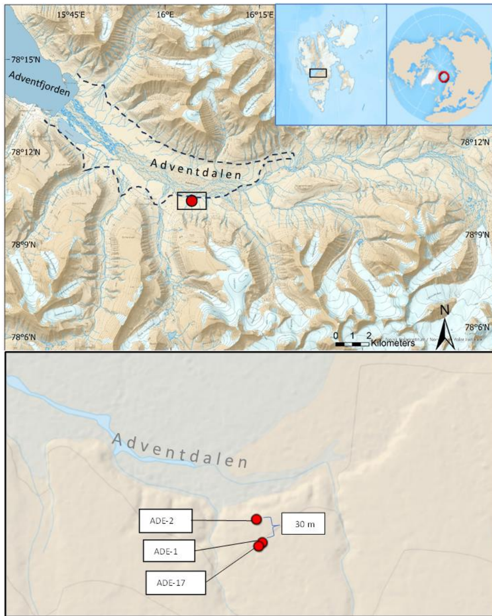
Figure 1: Location and detailed map of the ADE study site. The dashed line represents sea ingression limit at the early Holocene (Lønne and Nemec, 2004, drawn after Hodson et al., 2020). The map is provided with courtesy of the Norwegian Polar Institute.
