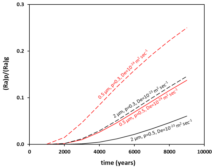
Figure 13: Simulations of diffusion from sediment clay grains into the pore space. (Ra)_p/(Ra)_g = Ra activity in pore space normalized to that in grain. See text for the diffusion coefficients used. Solid and dashed lines are for high and low porosity (0.5 and 0.3, respectively). See text for explanation about the simulations.
