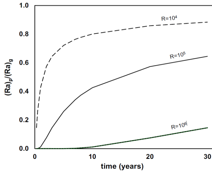
Figure 13: Simulations of diffusion from sediment grains into the pore space. (Ra)_p / (Ra)_g = Ra activity in pore space normalized to that in grain. Diffusion assumingly occurs through occasional liquidized ice along in-grain frozen nano-pores. De assumed 10-13 (see discussion in text). Retardation values are 10^4 - 10^6 to cover for fresh water at low T.
