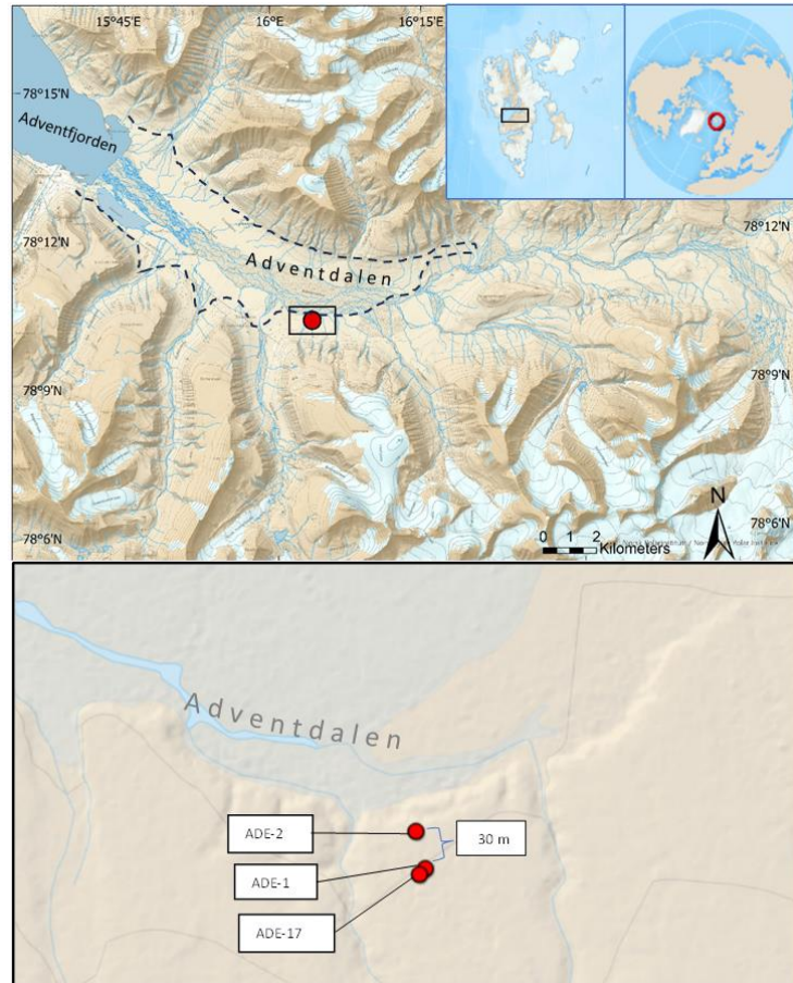
Figure 1: Location and detailed map of the ADE study site. The dashed line represents sea ingress limit at the early Holocene (Lønne and Nemec, 2004, drawn after Hodson et al., 2020). The map is provided with courtesy of the © Norwegian Polar Institute. All rights reserved.
