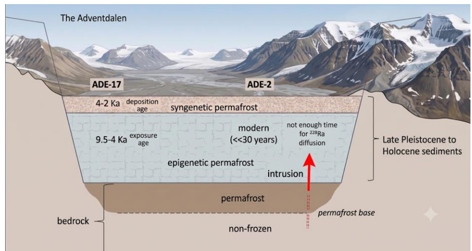
Figure 12. Conceptual model of ground ice versatility and residence times at the ADE site. See text for explanation. Note that locations of ADE-17 and ADE-2 are not to scale. In fact, they are located next to each other (within 30m).
