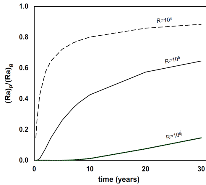
Figure 13: Simulations of diffusion from sediment grains into the pore space. (Ra)_p/(Ra)_g = Ra activity in pore space normalized to that in grain. Diffusion assumingly occurs through occasional liquidized ice along in-grain frozen nano-pores. De assumed 10-13 (see discussion in text). Retardation values are 10 4 -10 6 to cover for fresh water at low T.
