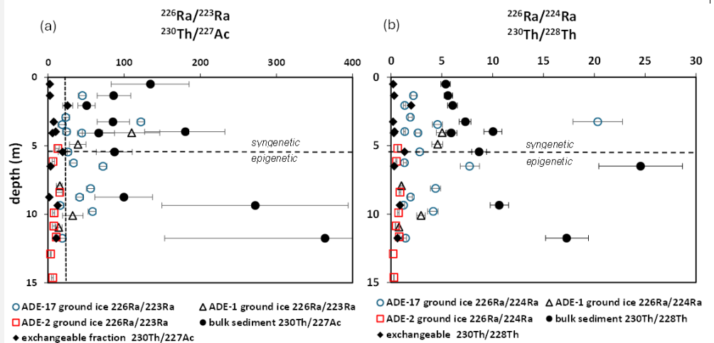
Figure 8: Radium isotope activities in ground ice and their parent ratios in bulk soil grains and on grain surfaces (exchangeable fraction). (a) ( ^{226}\text{Ra}/^{223}\text{Ra} ) AR and ( ^{230}\text{Th}/^{227}\text{Ac} ) AR . (b) ( ^{226}\text{Ra}/^{224}\text{Ra} ) AR and ( ^{230}\text{Th}/^{228}\text{Th} ) AR . The vertical dotted line in (a) indicates the natural ratio of ( ^{226}\text{U}/^{238}\text{U} ), parents of ^{226}\text{Ra} and ^{223}\text{Ra} , respectively. The dashed line as in Figure 3.
