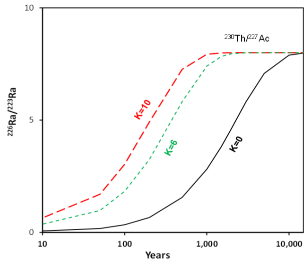
Figure 11: Simulations of the buildup of (^{226}\text{Ra}/^{223}\text{Ra})_{\text{ss}} in permafrost pore space with different adsorption coefficients ( K=0 means no adsorption). See text for further explanations.
