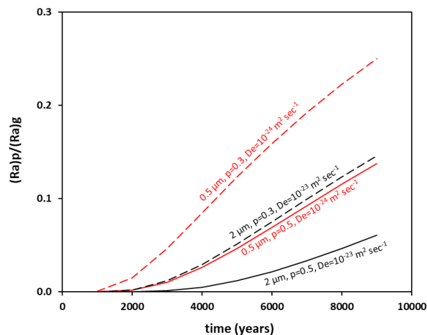
Figure 13: Simulations of diffusion from sediment clay grains into the pore space. (Ra)_p/(Ra)_g —Ra activity in pore space normalized to that in grain. See text for the diffusion coefficients used. Solid and dashed lines are for high and low porosity (0.5 and 0.3, respectively). See text for explanation about the simulations.
