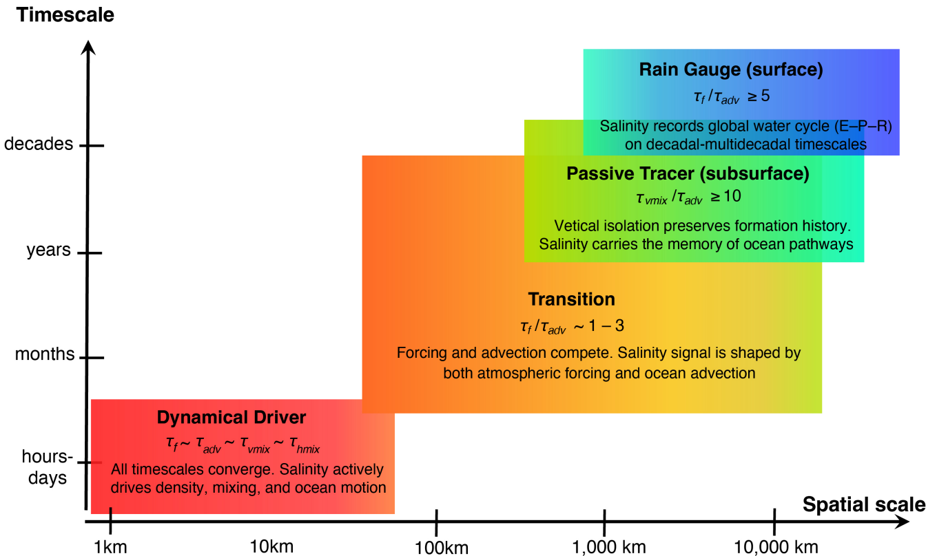
680 Figure 8. Salinity regime diagram. Four regimes from timescale competition (Table 3). Rain gauge (surface, cyan-blue): \tau_f/\tau_{adv} \geq 5 , forcing persists, pattern tracks E-P at basin-decadal scales. Passive tracer (subsurface, yellow-green): \tau_{vmix}/\tau_{adv} \geq
