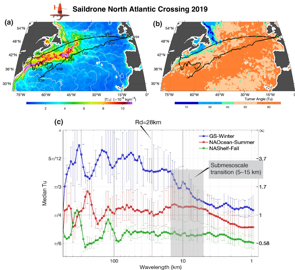
Figure 7. Thermohaline regime transition at submesoscales. (a) Sea surface density gradient magnitude and (b) Turner angle ( Tu ) from satellite observations with 2019 North Atlantic Sairdrone tracks overlaid (black lines). Tu less than 45^\circ (blue)
