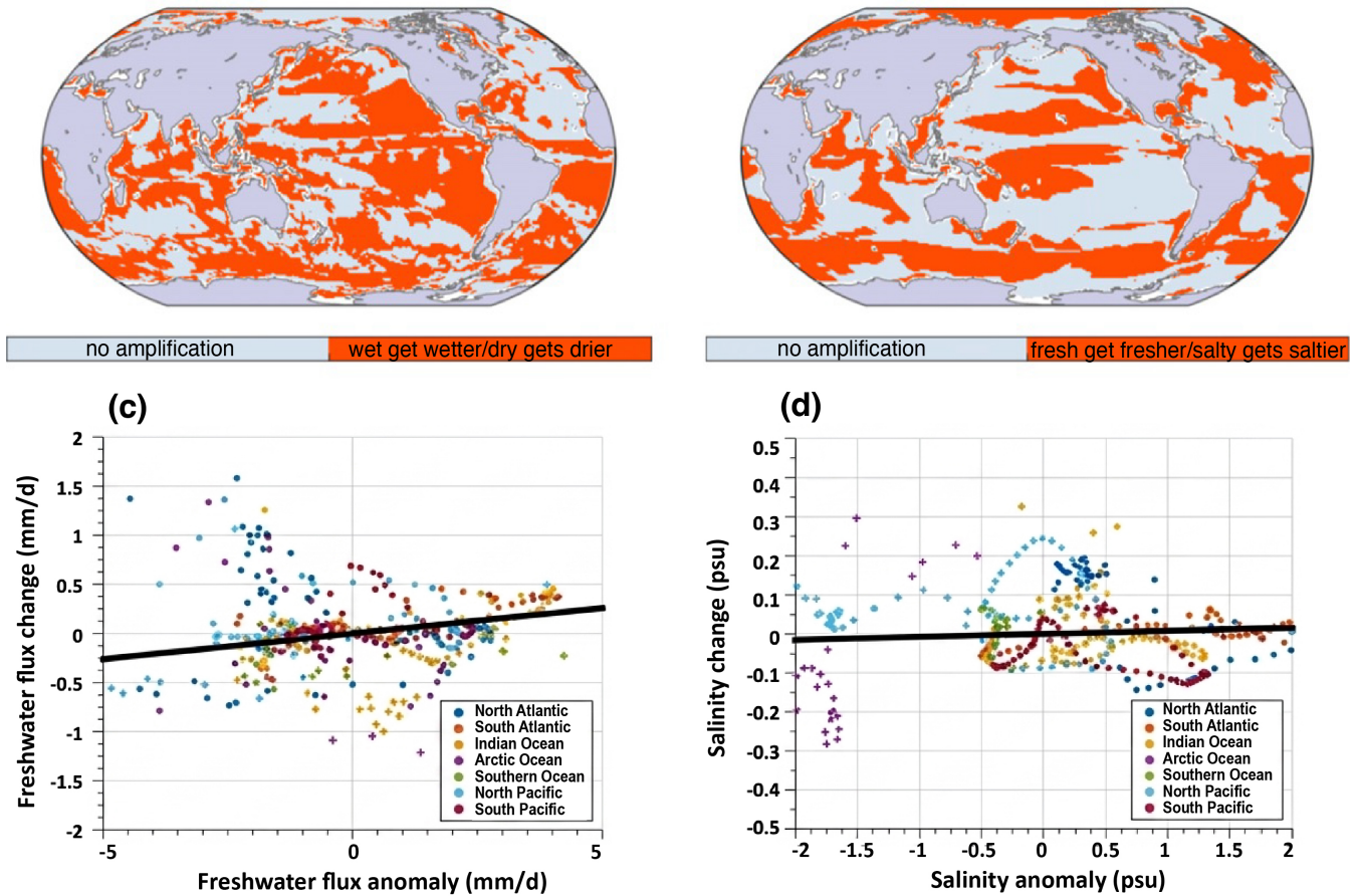
(a) Regions of amplification in the ocean water cycle
